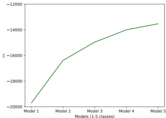
Figure 2.2: Log-Likelihood of Models (1-5 classes).
