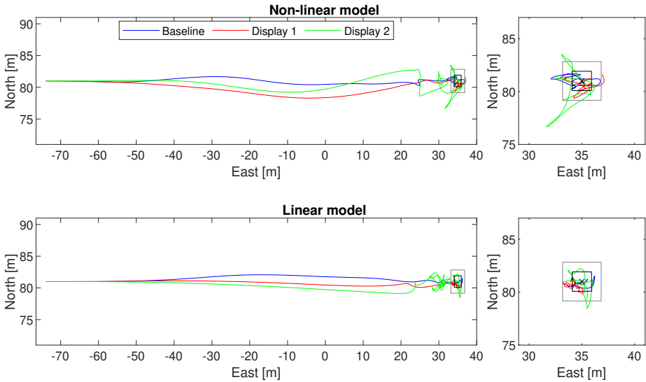
Figure 4.8: Ground tracks during full run (left) and during hover (right), one run per condition.
