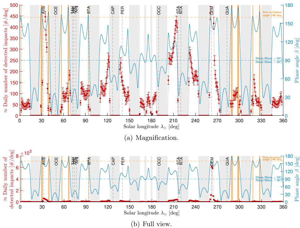
Fig. 22. Estimation of the temporal distribution of detected lunar impacts of LUMIO lunar CubeSat. On the left y-axis, the approximately daily number of impacts in 1 deg bins of solar longitude (the red dots joined with the dotted red line). KE \geq 10^{-6} kton TNT Equivalent, Earth equivalent. Results obtained from 1000 runs. On the right y-axis, the phase angle \beta (the blue solid line). The horizontal dashed blue line marks the phase angle at which Moon illumination is equal to 50%. The horizontal dashed orange line marks the phase angle corresponding to the Sun exclusion angle. The gray shaded areas highlight the epochs in which monitoring is unfeasible due to the elevated Moon illumination. The orange shaded areas highlight the epochs in which monitoring is unfeasible due to the large quantity of straylight coming from the Sun. The vertical dashed black lines are the solar longitudes at which activity periods of some major showers peak.
