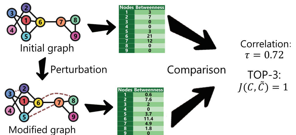
Fig 3. Perturbation analysis for the betweenness centrality: an example.
