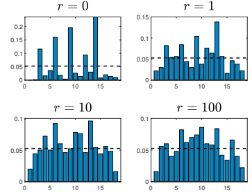
Fig. 4. Relative frequency of a point being reached from \alpha_1(y) , for each point in the elliptic curve E(\mathbb{F}_{17}) , indexed over \{1, \dots, |E(\mathbb{F}_{17})|\} .
