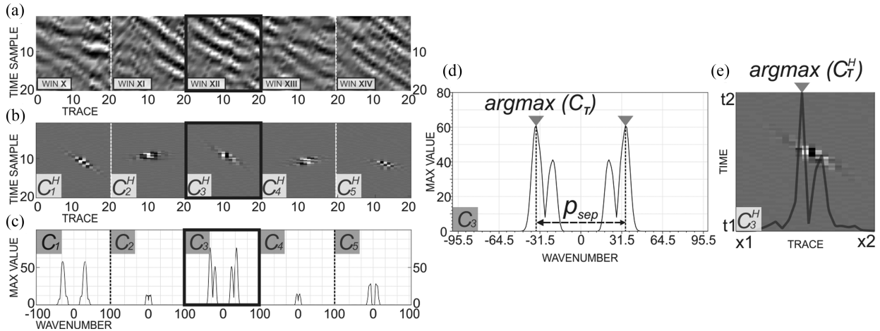
Figure B1. Curvelet parametrization of a single VSG. (a) Coherent events extracted from the selected windows. The roman numbers refer to the position of the VSG along receiver line 6. For each VSG, we choose a single window including a coherent event (referred to as the target window and marked by a bold line) and two windows from the left and right adjacent VSG positions. Note that for the configuration shown in this figure, the target window is WIN XII and the remaining windows are input to the denominator in eq. (B2). (b) Inverse curvelet transform of wedges associated with windows in (a). (c) Maximum values of the forward curvelet transforms narrowed to part of the data falling in the chosen window. (d) Sketch illustrating parameters used to obtain W_{P2} . (e) Sketch illustrating parameters used to obtain W_{P1} . For parameter definition, see the description of eqs (B3) and (B4).
