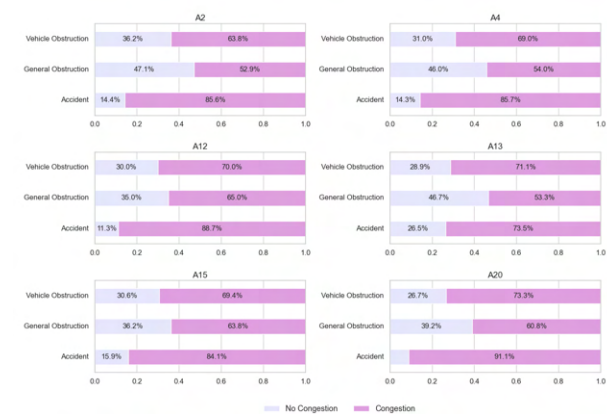
Fig. 9: Percentage of matched incidents with significant congestion per incident category on studied motorways (August-December 2019).
