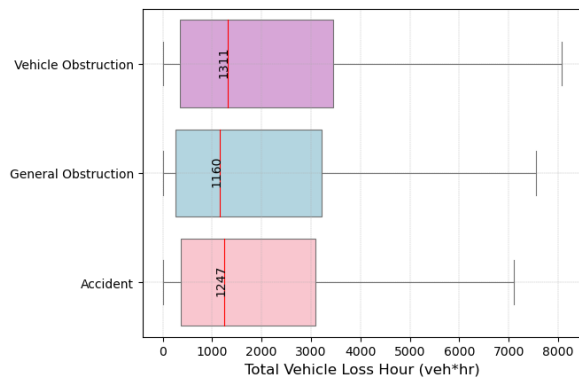
Fig. 10: Estimated total Vehicle Loss Hour (VLH) for different incidents (August-December 2019).
