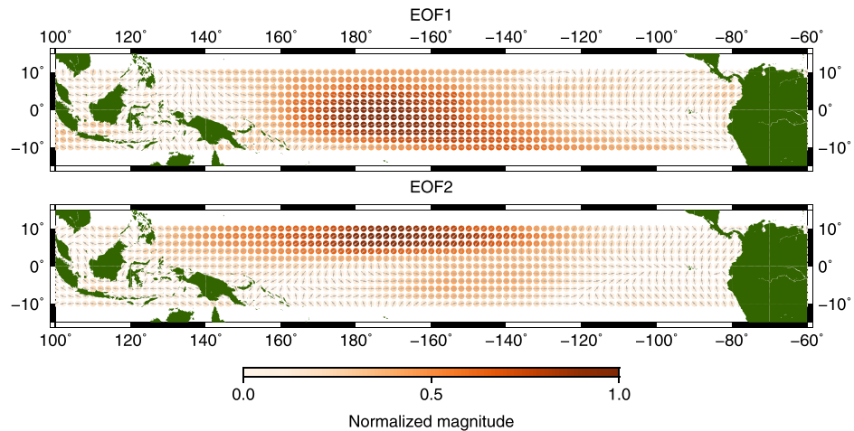
Figure 5. The first two EOFs corresponding to the PCs of the wind stress. The colors indicate the intensity of the wind stress and the vectors the direction.
