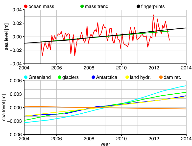
Figure 11. (top) In red the sea level time series (m) for the whole TAS region, after removing the contributions of the regressed PC1&2 and DMI indices, the nodal cycle and the annual and semiannual cycles. In black the sum of the mass fingerprints. (bottom) The fingerprint time series of Greenland, glaciers, Antarctica, dam retention and land hydrology respectively in light blue, green, blue, yellow, and orange.
