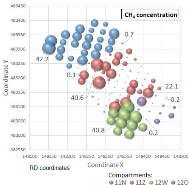
FIGURE 3: Spatial distribution of \text{CH}_4 concentration (vol.%) in the extraction wells - March 2020. The size of the symbol is indicative of \text{CH}_4 concentration.
