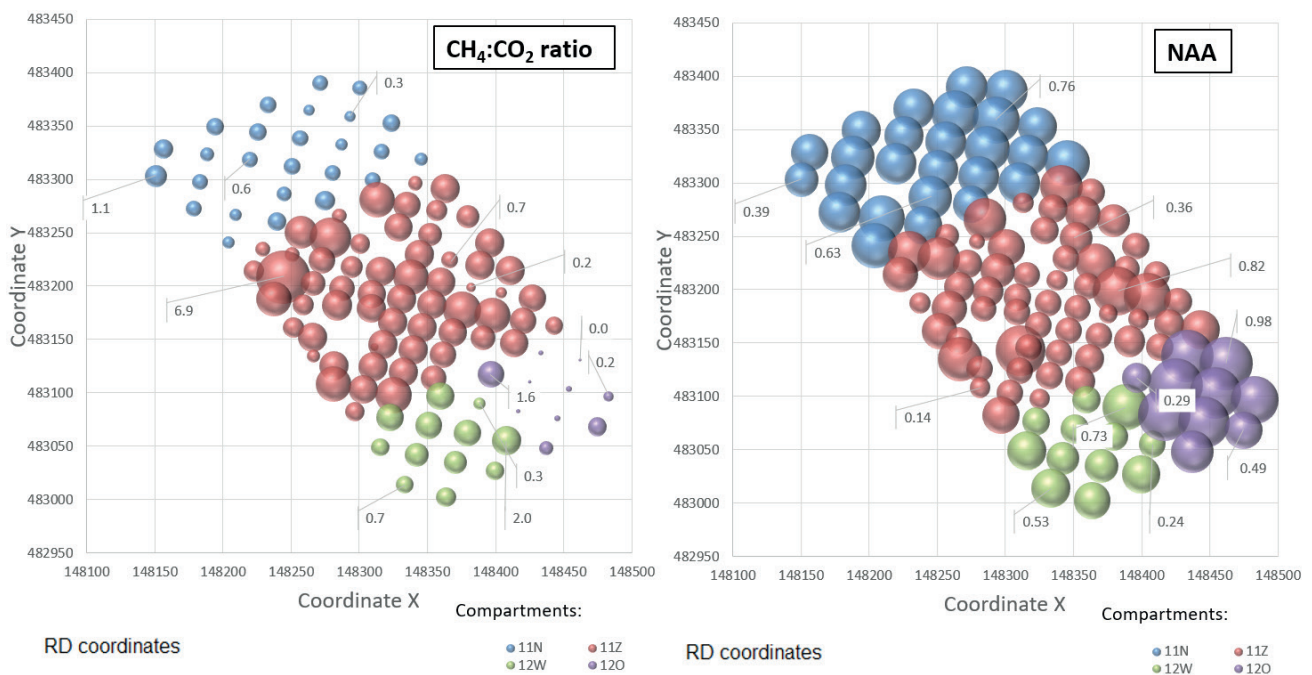
FIGURE 4: Spatial distribution of the ratio \text{CH}_4 to \text{CO}_2 in the extraction wells (left) and percent of anaerobic activity (right) - March 2020. The size of the symbol is indicative of the ratio \text{CH}_4 to \text{CO}_2 .
