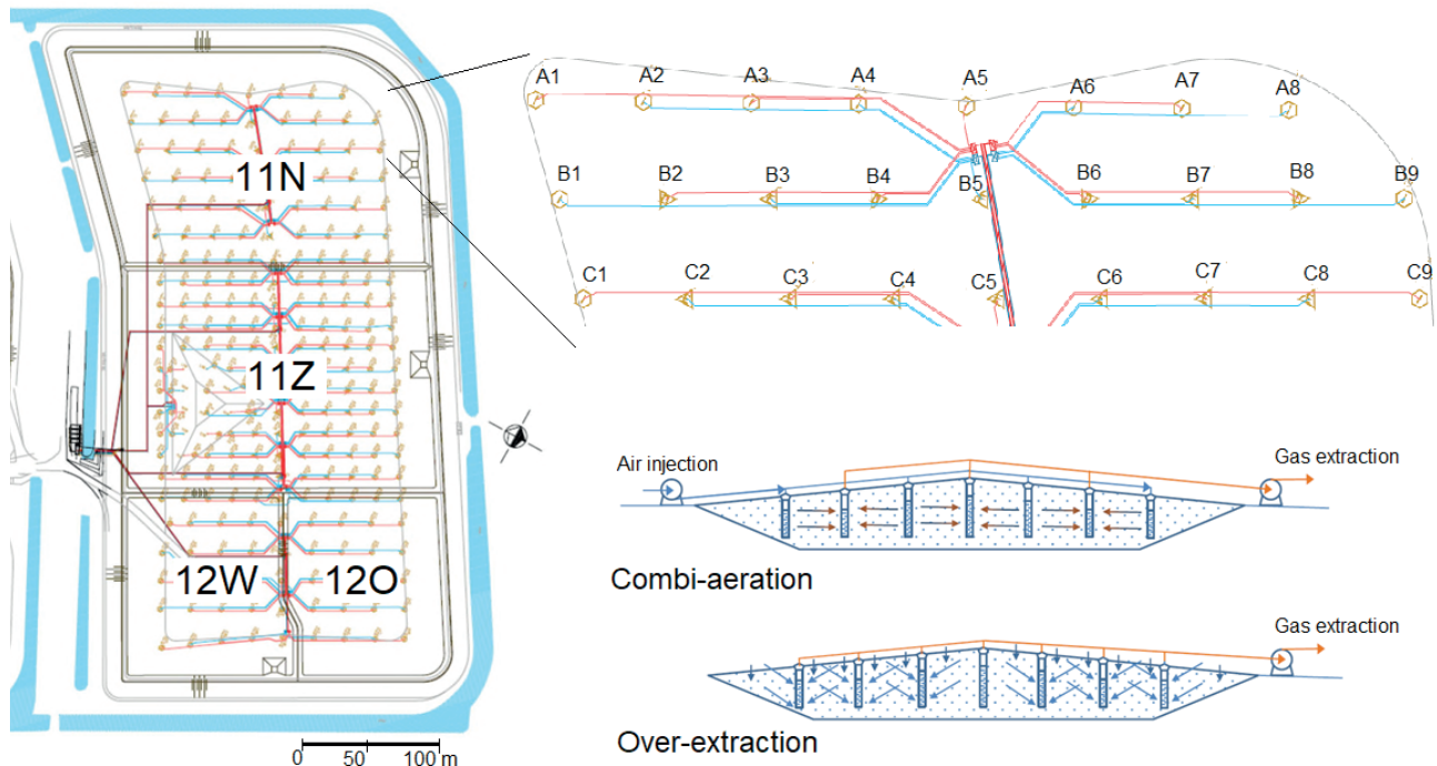
FIGURE 2: Network of aeration wells, systematics of well labeling and a schematic representation of combi-aeration and over-extraction.
