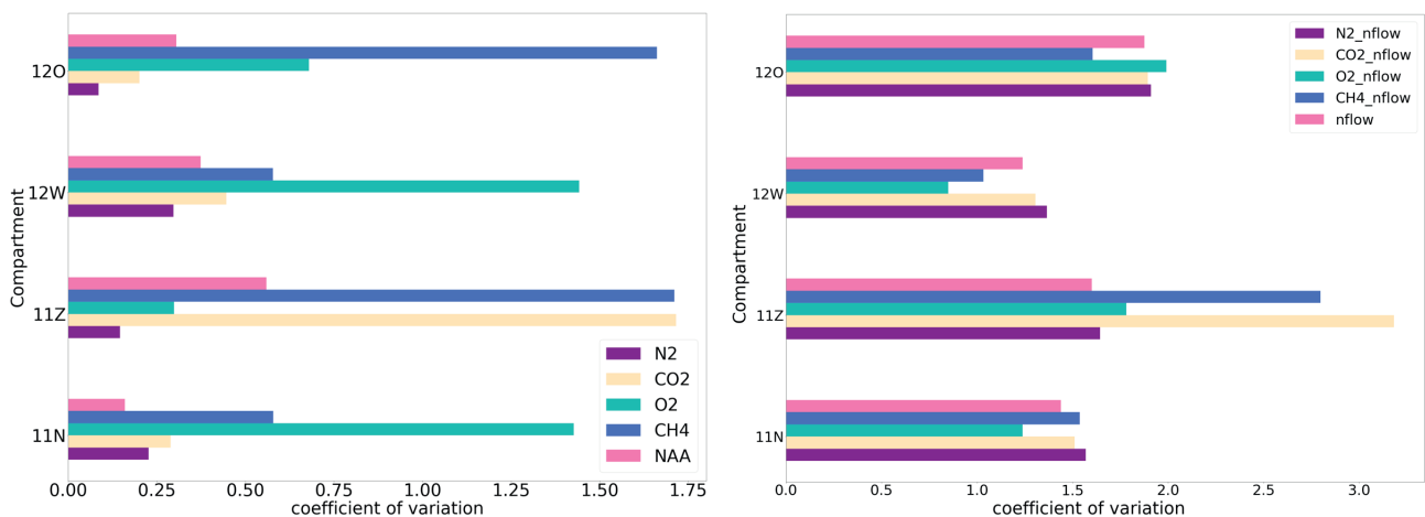
FIGURE 5: Coefficient of variation for the concentration of \text{CH}_4 , \text{CO}_2 , \text{O}_2 , and \text{N}_2 , and normalized aerobic activity (NAA) (left) and for flow rate, and flow rates of \text{CH}_4 , \text{CO}_2 , \text{O}_2 , and \text{N}_2 in the gas extraction wells - March 2020.
