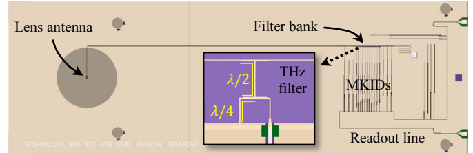
Fig. 1. Prototype chip of a sparsely sampled spectrometer in the band 300-400 GHz. In the inset one can observe one example of an “I-shaped” THz bandpass filter coupling power from the through-line to an MKID behind it.
