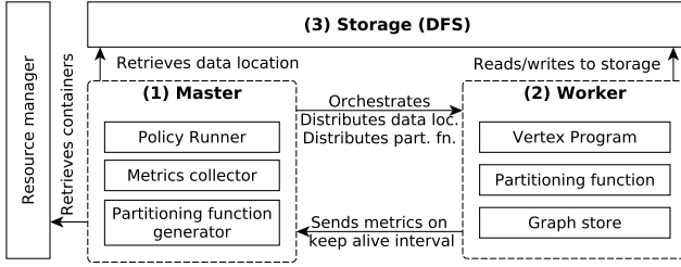
Fig. 4. Overview of the JoyGraph EGAP architecture.
