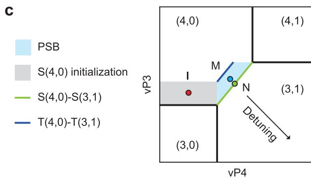
Fig. 1 Device and charge stability diagram. a False-colored scanning electron microscope image of the device. The green, purple, and brown gates correspond to plunger/accumulation, barrier, and screening gates, respectively. The lower channel is used for defining the right and left quantum dots under the plunger gates P3 and P4 (lower panel). A micromagnet is fabricated on top of the fine gate stack. The right quantum dot in the upper channel is used as a charge sensor quantum dot. The right bath for the charge sensor is connected to a radio frequency tank circuit. The white circles indicate where quantum dots are formed. The scale bar is 200 nm. b Charge stability diagram for the four-electron configuration. V_{\text{R}} is the reflectometry signal from the charge sensor. The v\text{P4} voltage sweep is performed from right to left so that the triplet (3,1) state is latched in the spin blockade regime. The dashed white trapezoidal region indicates where the latching due to PSB occurs. The point O (black circle in the (3,1) configuration) indicates the charge symmetry point where the qubit operation is performed. c Zoom in schematic stability diagram around the (4,0)–(3,1) charge degeneracy point. The red, blue, and green points show the plunger gate configurations for initialization (I), measurement (M), and inter-dot transition (N). The right blue area shows the configuration where PSB occurs. The gray area shows that energy-selective tunneling to S(4,0) occurs. The green (blue) line around the border of the PSB region shows the inter-dot transition for the singlet (triplet) states. The detuning is defined as v\text{P4}-v\text{P3} .
