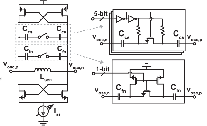
Fig. 3 Schematic of the digitally controlled oscillator (DCO)
