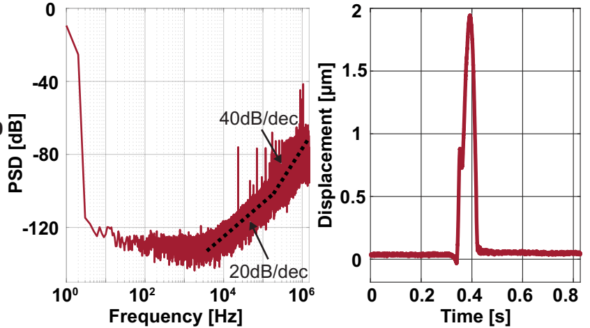
Fig. 5 Output power spectral density (PSD) vs. Frequency [Hz] and Fig. 6 Sensor response to touch (Displacement [ \mu\text{m} ] vs. Time [s])
