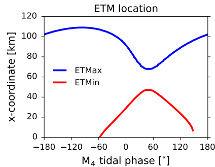
Figure 13. Sensitivity of the location of the ETM to varying external M_4 tidal phases in the Scheldt Estuary. The blue and red lines indicate a maximum and minimum in the sediment concentration in the model domain respectively.
