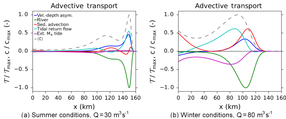
Figure 12. The five most important tidally averaged sediment transport contributions, rescaled with the maximum transport. Negative values indicate export, while positive values indicate import. Total net transport of all terms added yields zero. The scaled tidally averaged depth-averaged sediment concentration (grey dashed line) is plotted in the background for reference. Parameter values corresponding to the Scheldt Estuary.
