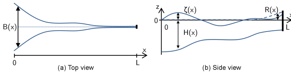
Figure 2. Model domain. The model is two-dimensional in the along-channel ( x ) and vertical ( z ) directions and is width-averaged. The depth and width are allowed to vary smoothly with x .
