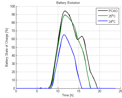
Fig. 5: Battery evolution during the day
