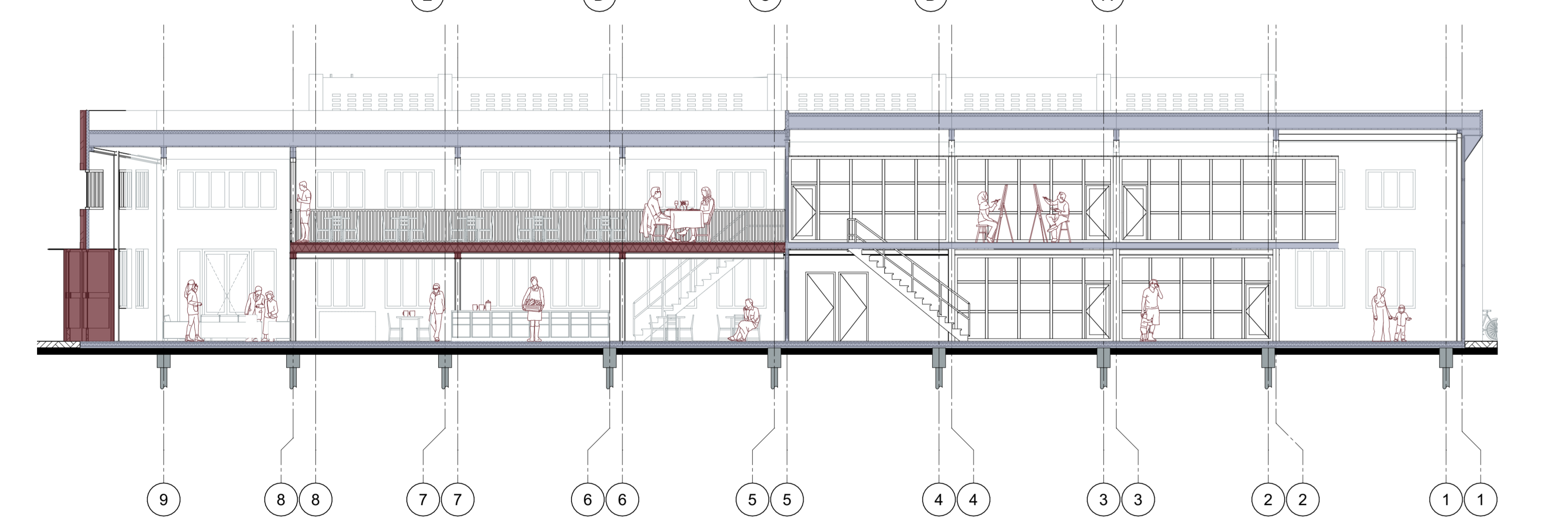
NORTH BUILDING EAST - WEST SECTION 1:100
