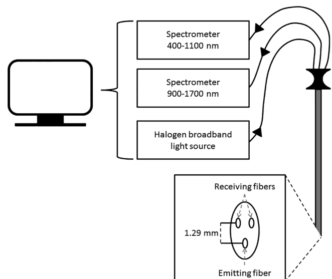
FIGURE 1 Schematic of the measurement setup. The setup includes two spectrometers and a halogen broadband light source. The measurement needle contains three fibers, one to transport light to the tissue and two to transport the light from the tissue to the two spectrometers
