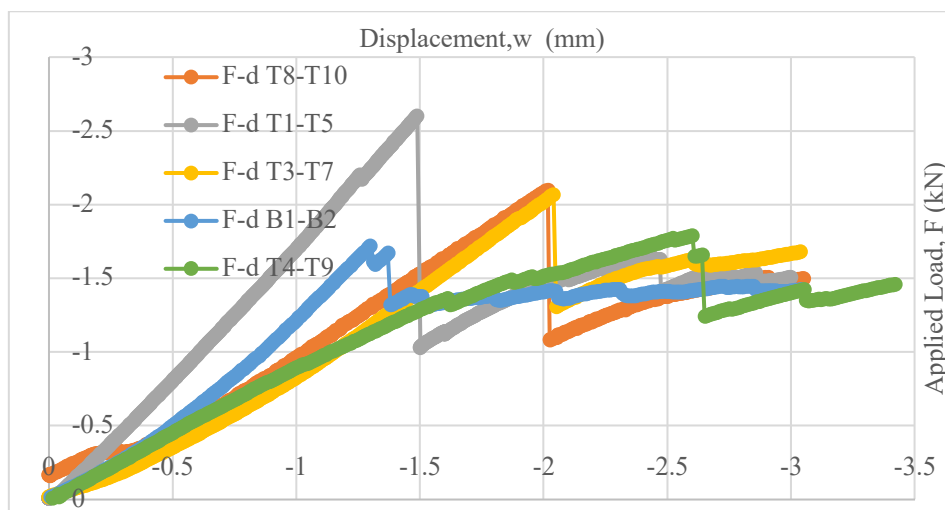
Figure 11. Load-Displacement curves. Static component tests.
