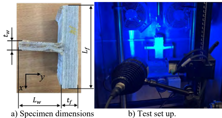
Figure 5. Component tests.
