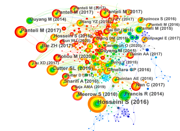
Fig. 12. Cited author analysis for resilience assessment.
