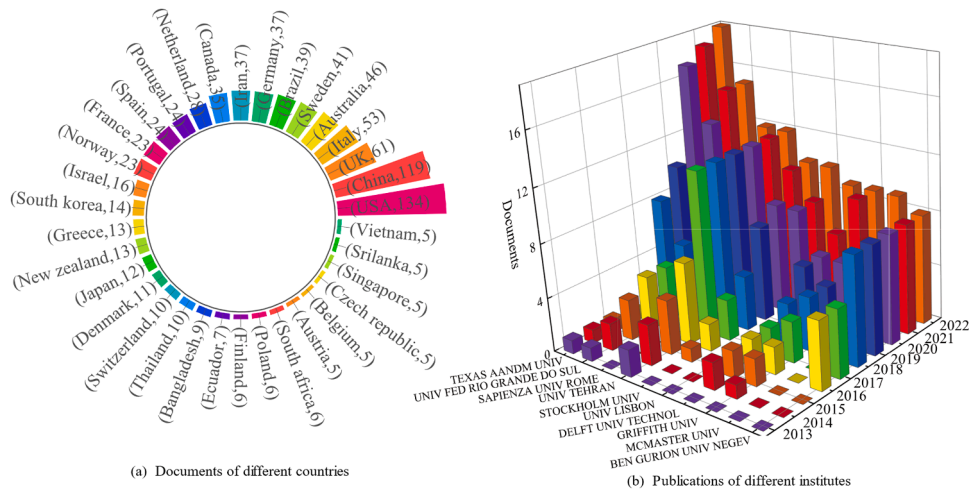
Fig. 14. Publication count of most relevant institutes and countries.
