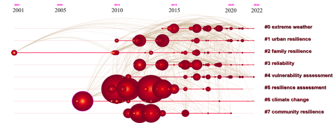
Fig. 11. Timeline for keywords clusters.
