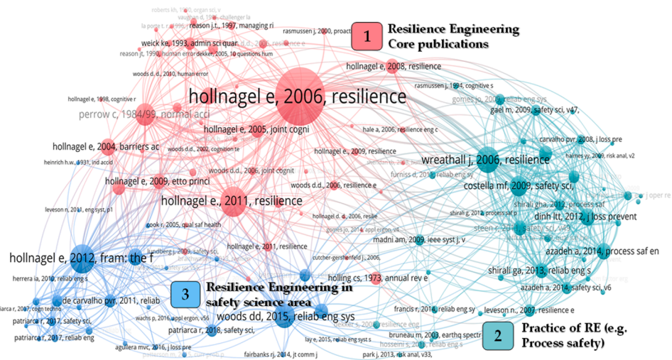
Fig. 10. Documents co-citation analysis of resilience management (the label indicates the first author and the publication year, with the sublabel indicating the source of the document).
