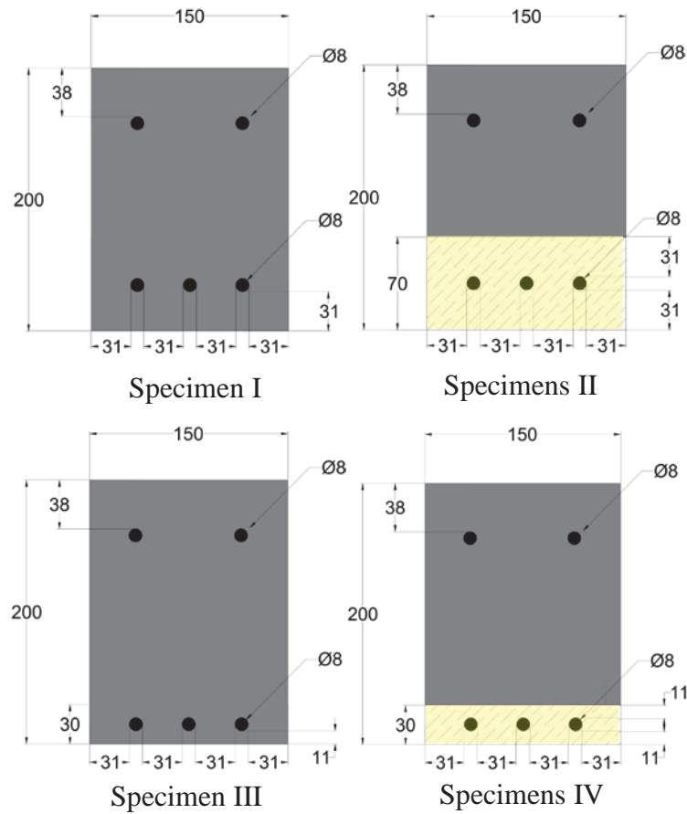
Figure 1: Cross sections of beams; concrete = grey, SHCC = yellow (units in [mm])
