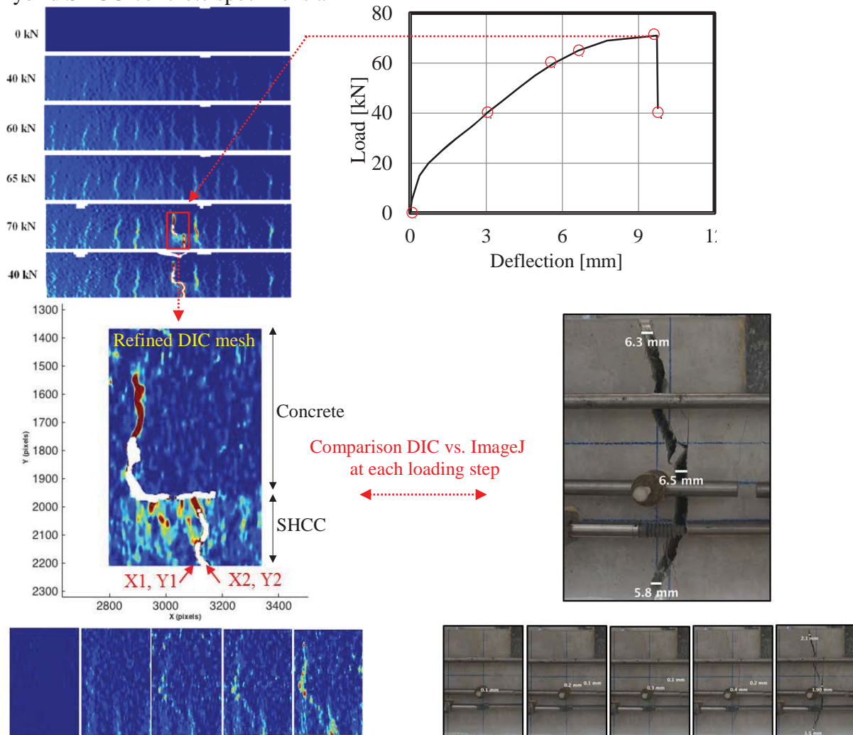
Figure 5: Verification of DIC measurement with ImageJ measurements (the crack opening at each loading step was obtained by equation (1) from DIC)
