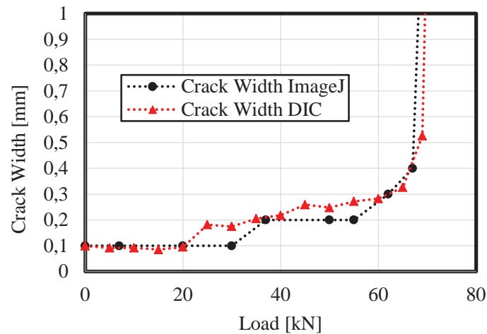
Figure 6: Verification of DIC for capturing crack opening, comparison with ImageJ analysis
