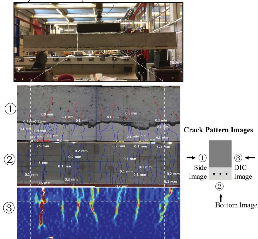
Figure 7: Damage at the failure in the Specimen 2-II beam
