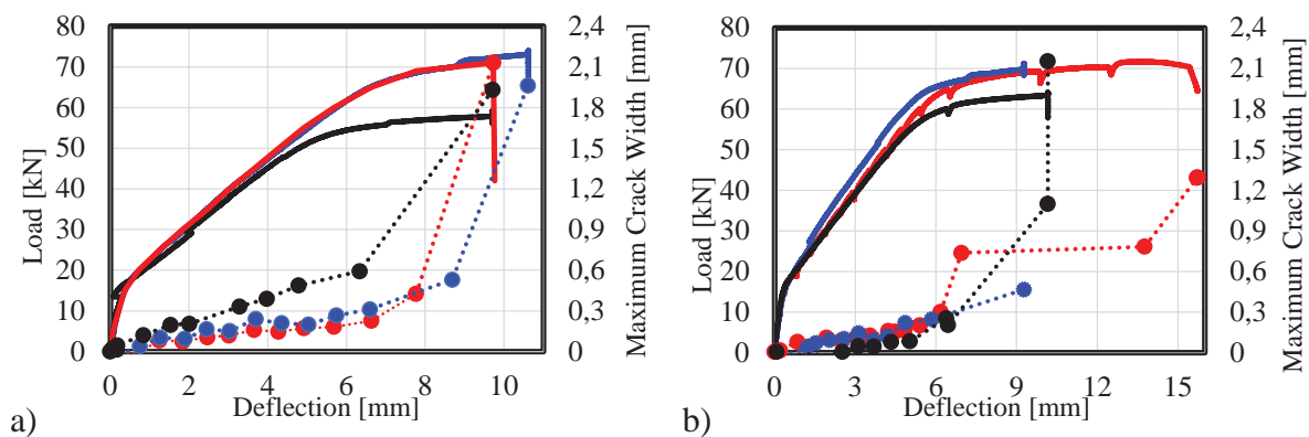
Figure 8: Load-deflection relation and load-maximum crack width relation in beams with a SHCC layer of a) 70 mm and b) 31 mm (black = reference beam, red = pure SHCC layer and blue = SHCC + self-healing)
