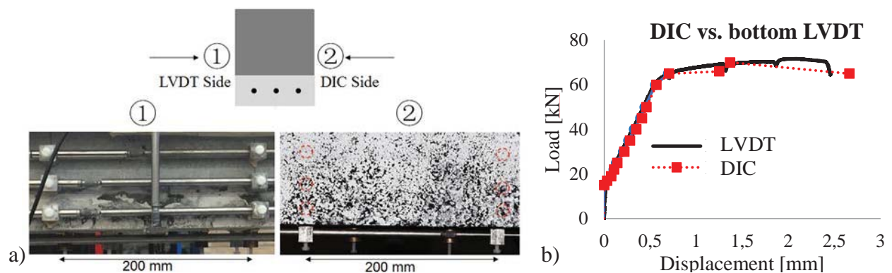
Figure 3 a) Verification of DIC over the length of 200 mm measured by LVDT b) Results
