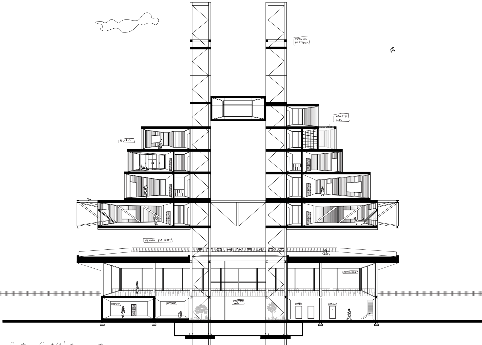
Section East West perspective
