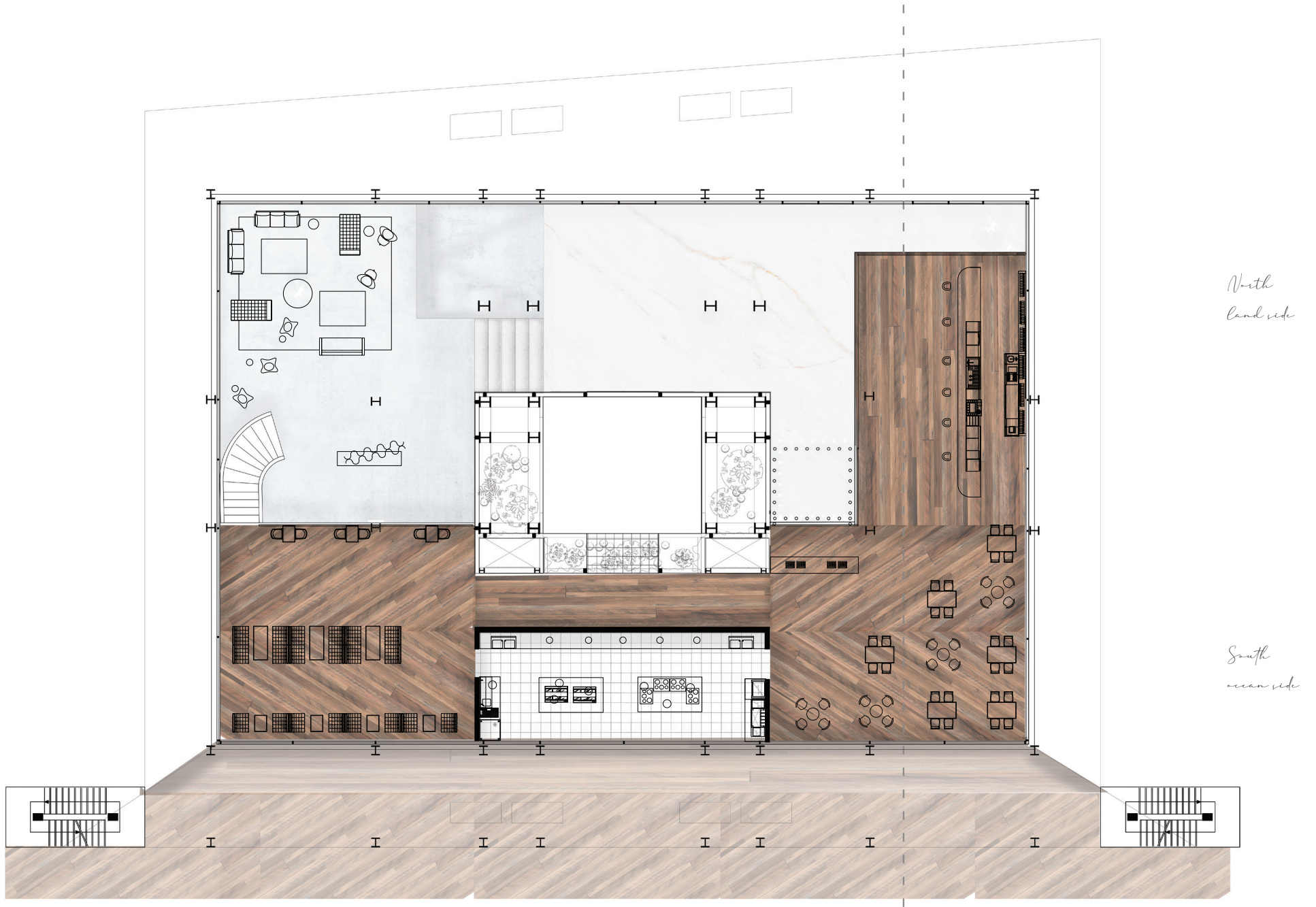
Ground floor - restaurant materials.
