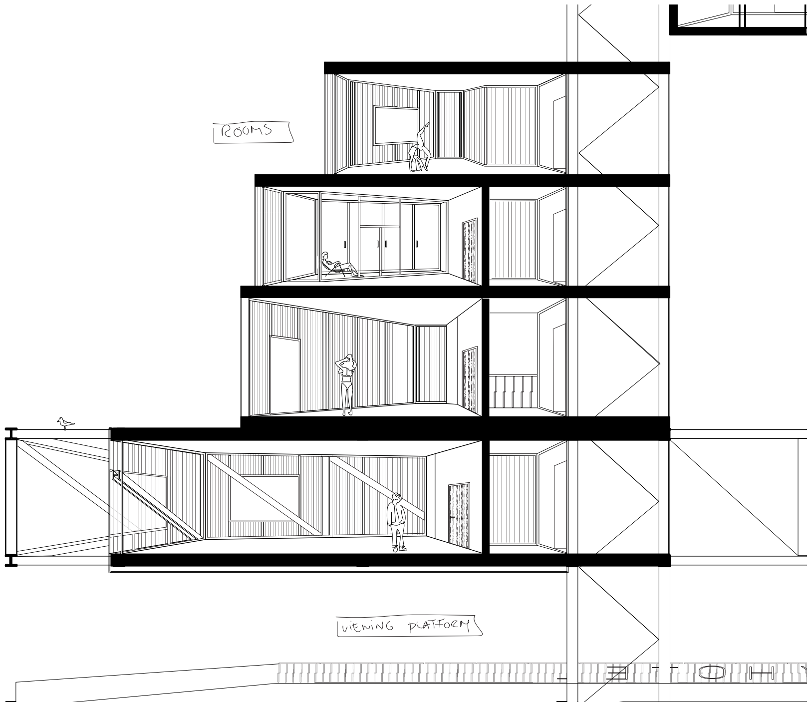
Section East West rooms East
