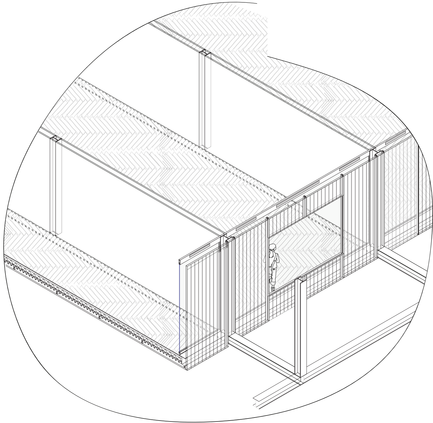
isometric section room facade window opening
