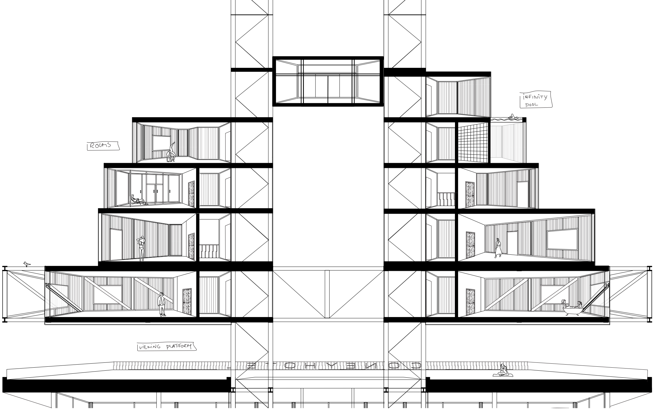
Section East West rooms - top
