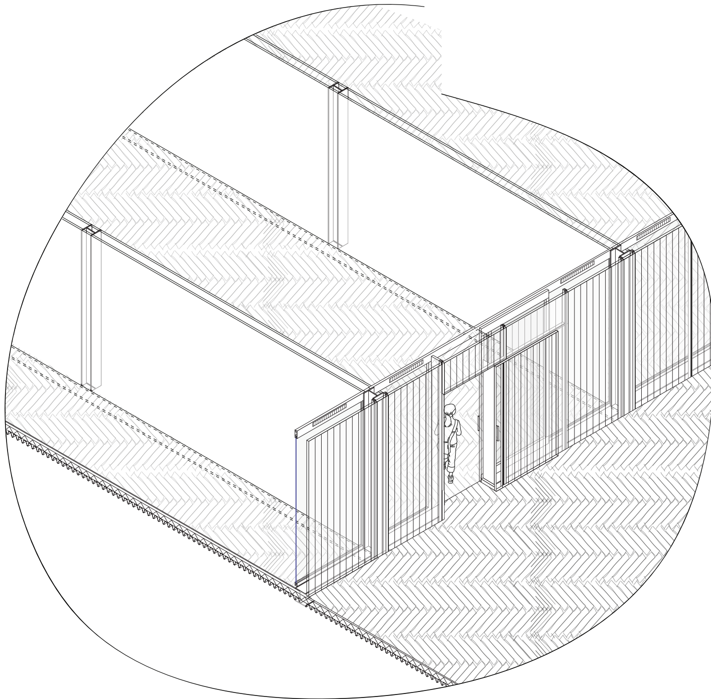
isometric section room facade sliding door
