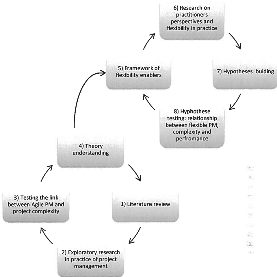
Figure 1-3: Research design
