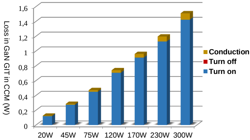
Figure 5.3 Loss breakdown of high voltage GaN GIT in CCM
