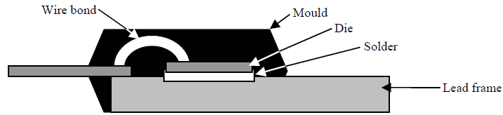
Figure 4.19 Cross-section of a conventional packaging approach [4-17]
