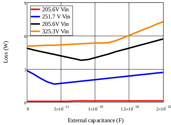
Figure 6.5 Effects of external capacitance on loss GaN GIT
