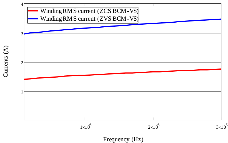
Figure 5.42 Influence of frequency on RMS current in inductor winding
