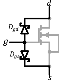
Figure 4.4 Equivalent diodes in circuit model of GaN HEMT
