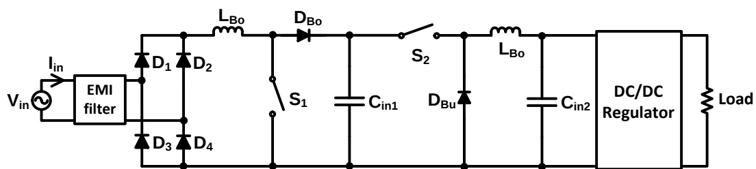
Figure 3.16 Boost-cascade-buck as PFC preregulator
