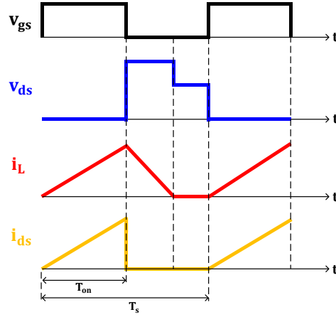
Figure 5.8 Representative waveforms of DCM (theoretical)
