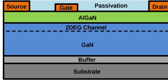
Figure 2.2. Basic structure of lateral GaN transistors
