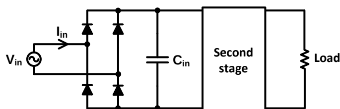
Figure 3.1 Capacitor-filtered AC/DC converter
