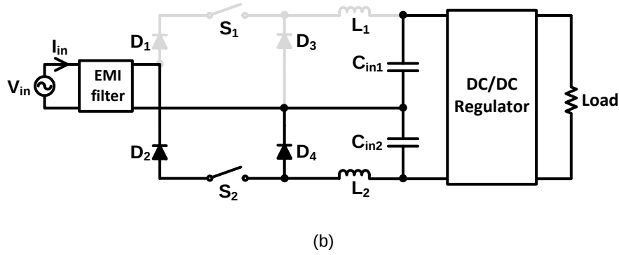
Figure 3.13 Operation of bridgeless buck PFC converter during the positive line voltage (a) and negative line voltage (b).
