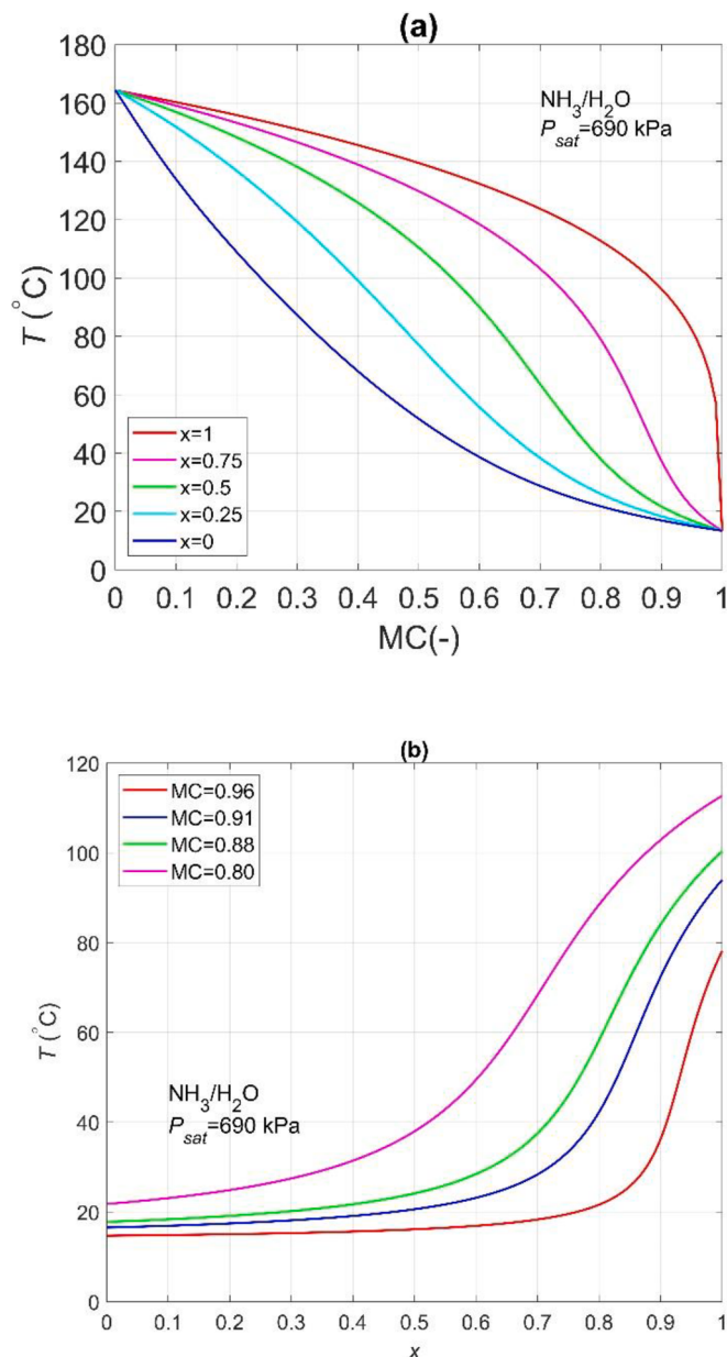
Fig. 1. (a) Temperature glide of \text{NH}_3/\text{H}_2\text{O} with varying mass concentrations. The equilibrium temperatures of bubble point, dew point and three vapor qualities are indicated. (b) Equilibrium temperature as a function of vapor quality for different mass concentrations.
