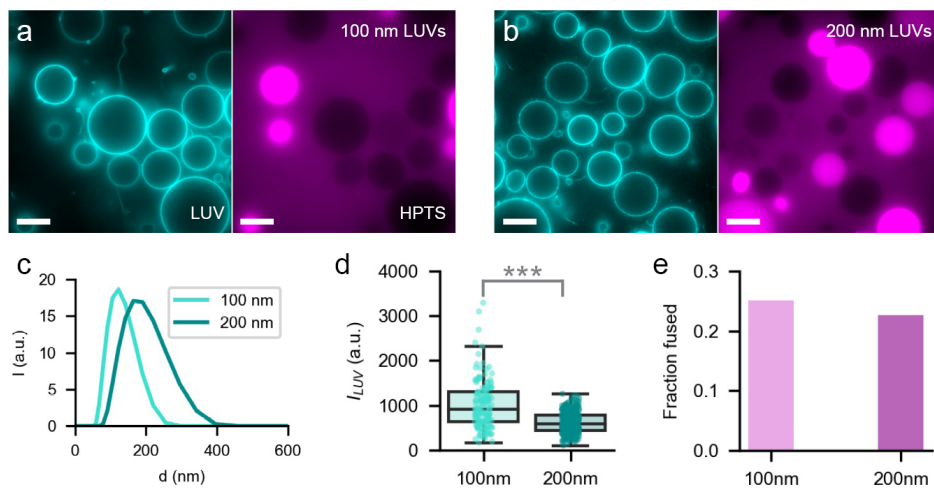
Figure 7.11: Fusion assays using LUVs of different sizes. Fusion was performed by pre-incubation with 1\mu M chol-DNA and at hypotonic conditions of -25mOsm . (a-b) Epifluorescence images of unlabelled DOPC GUVs incubated with LUVs labelled with 0.05 % Rhodamine DOPE (mol/mol). LUVs contained 10mM HPTS to visualize content mixing. Scale bar is 20\mu m in all images. (a) 100nm LUVs. (b) 200nm LUVs. (c) DLS results for DOPC LUVs produced by extrusion with a membrane pore size of either 100nm (cyan) or 200nm (dark cyan). Data presented is the intensity distribution of particle sizes. (d) Population analysis of LUV intensity on the GUV membrane (***) p < 0.001 ). Each point represents an individual GUV. (e) Fraction of fused GUVs calculated from the HPTS ratio inside versus outside GUVs.
