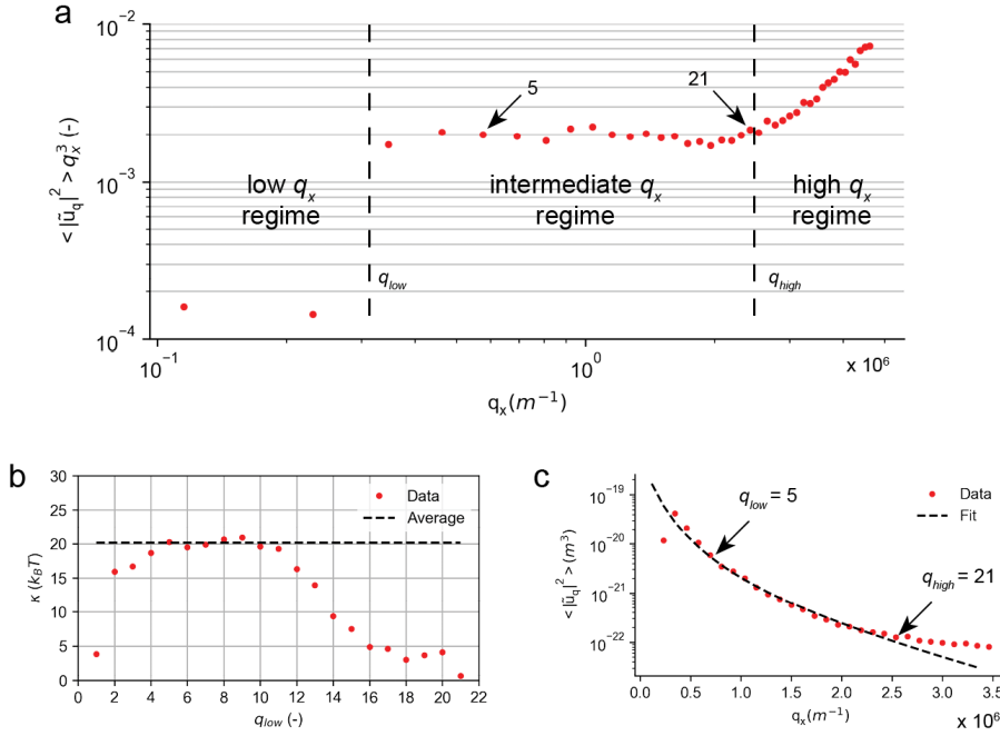
Figure 6.6: Example VFA analysis for a DOPC vesicle. Fluctuation spectrum and fitting for a DOPC vesicle with a radius of 8\ \mu\text{m} made by electroformation and imaged in epifluorescence with 5 ms exposure time. (a) Scaling of the variances with wave number q_x reveals three different regimes: only the intermediate regime where variances scale with q_x^{-3} is used for fitting. The lower and upper cut-off modes, q = 5 and q = 21 , are indicated. (b) Fitting results in values of \kappa as a function of q_{low} . It can be seen that from mode 5 to 11, \kappa minimally depends on q_{low} . Averaging \kappa over these modes yields \kappa = 20k_B T (black dashed line). (c) Final fitting results using \kappa = 20k_B T , \sigma = 2.6 \cdot 10^{-9} \text{ N/m} , q_{low} = 5 and q_{high} = 21 .
