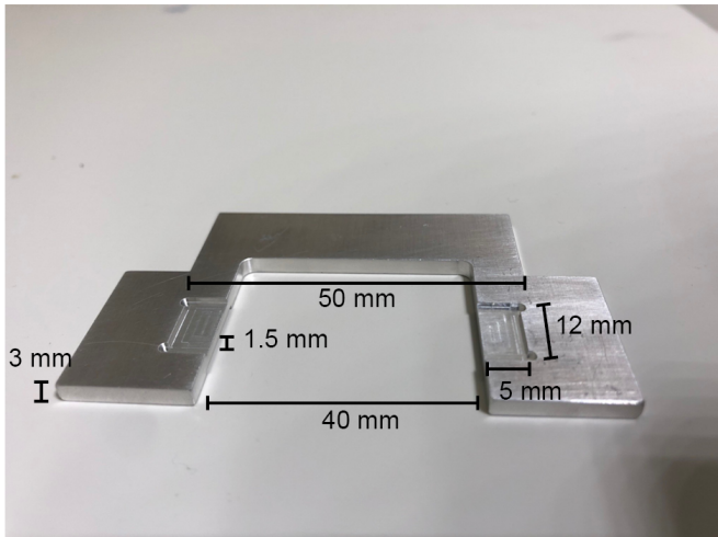
Figure 6.15: Sample chamber for MPA measurements. Aluminum spacer used for constructing micropipette aspiration chamber. Slots seen here on top are made to fit a glass slide, which serves as the top of the chamber. Similar slots are present on the bottom to insert the bottom coverslip.
