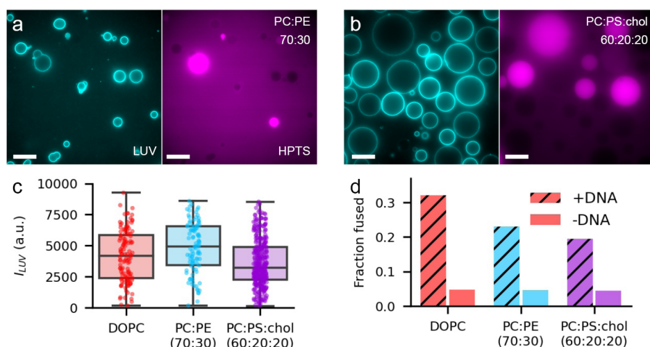
Figure 7.12: Fusion using GUVs with different membrane compositions. (a-b) Epifluorescence images of GUVs in content mixing assays. Both GUVs and 200 nm DOPC LUVs (cyan) were incubated with 1\mu\text{M} chol-DNA prior to the fusion step. LUVs encapsulated 10 mM HPTS (magenta) as an indicator for membrane fusion. Scale bar is 20\mu\text{m} in all images. (a) GUVs were produced from a lipid composition consisting of 69.5% DOPC, 30 % POPE and 0.5 % Atto 488 DOPE. (b) GUVs were formed from a lipid composition of 59.5 % DOPC, 20 % DOPS, 20% cholesterol and 0.5% Atto 488 DOPE. (c) LUV intensity measured on the GUV membrane. Each point represents an individual GUV. (d) Fraction of fused vesicles for different GUV membrane compositions tested. Dashed bars indicate experiments including an incubation step of 1\mu\text{M} chol-DNA for both GUVs and LUVs, plain bars represent a control experiment where no chol-DNA was added in the incubation step.
