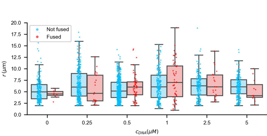
Figure 7.16: GUV radii of fused and non-fused populations with varying DNA concentration. GUV radii of fused and non-fused vesicles at different DNA concentrations as shown in fig. 7.3. GUVs are considered fused when the HPTS intensity ratio was larger than 1.05. Each data point represents an individual GUV.
