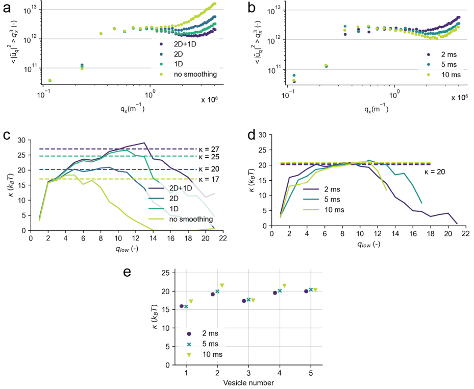
Figure 6.7: Influence of image processing and exposure time on VFA. (a) Plateau plot for one video of a fluctuating DOPC vesicle with a radius of 8\mu\text{m} imaged in epifluorescence with 2 ms exposure time, treated with different image processing options prior to membrane detection. ‘2D’ is two-dimensional smoothing, ‘1D’ is one-dimensional smoothing, ‘2D+1D’ is both smoothing procedures combined, and ‘no smoothing’ means contour detection was performed in the unprocessed image. Values are plotted against the wave number. (b) Plateau plot for the same vesicle imaged with exposure times of 2, 5 and 10 ms, analysed with two-dimensional smoothing, plotted against the wave number. (c-d) Dependence of \kappa on q_{low} for the fluctuation spectrum in (a) and (b). Averaged values of \kappa obtained from the plateaus are indicated with dashed lines. Values are plotted against the mode number. (e) Bending rigidities obtained for five vesicles with radii between 6 and 9\mu\text{m} imaged with different exposure times. Values were shifted and placed arbitrarily on x-axis for ease of view.
