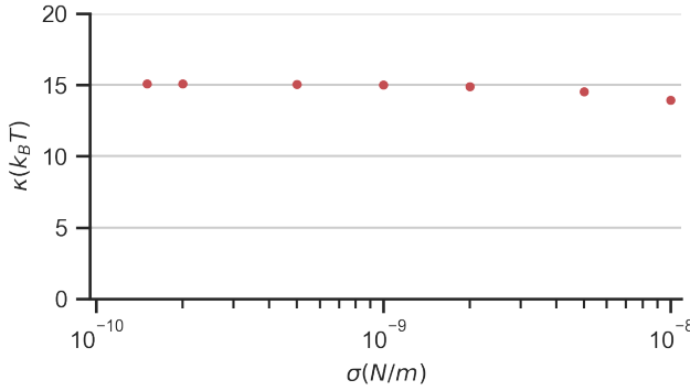
Figure 6.13: Effect of membrane tension on the fitting of bending rigidity. A theoretical fluctuation spectrum was calculated using \kappa = 15k_B T and \sigma = 10^{-9} N/m . Fitting the spectrum using a range of fixed \sigma values resulted in bending rigidities close to 15k_B T (red dots), with at maximum 1k_B T difference.
