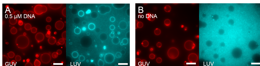
Figure 5.10: Binding of LUVs at different DNA concentrations. Images are epifluorescence images of Atto488 DOPE incorporated in the GUV membrane (red) and Atto 655 DOPE in the LUV membrane (cyan). Scale bar is 20\ \mu\text{m} in all images. (A) At 0.5\ \mu\text{M} cholesterol-DNA, LUVs bound to the GUV membrane. (B) No membrane localization was observed in absence of cholesterol-DNA.
