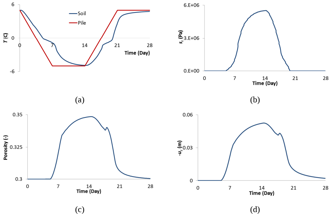
Fig. 9 Time histories: (a) soil temperature, (b) cryogenic suction, (c) porosity, (d) vertical displacement.
