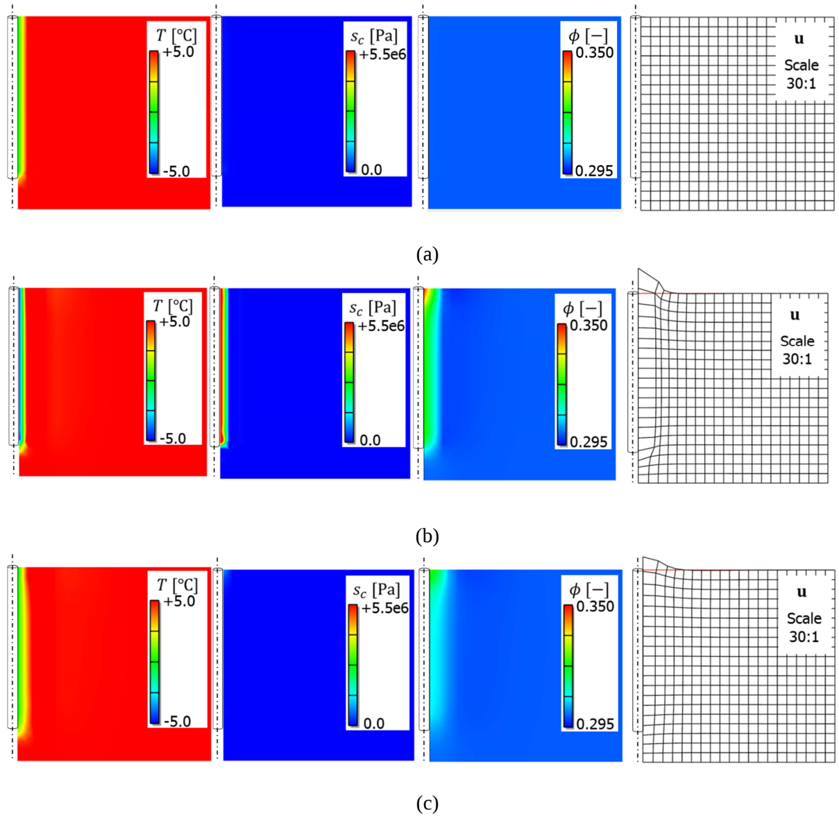
Fig. 8 Computational results for temperatures, cryogenic suctions, porosities, and deformed mesh: (a) just before freezing ( t = 5 \text{ days} ), (b) during freezing ( t = 14 \text{ days} ), (c) just after freezing ( t = 19 \text{ days} ).
