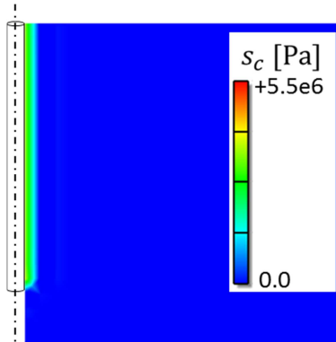
Fig. 12 Standard FEM with 400 elements. Cryosuction at Day 14.
