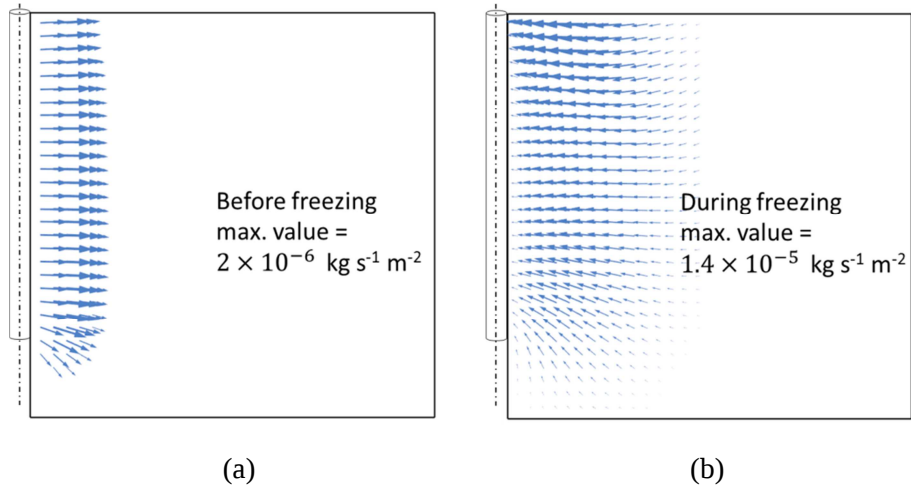
Fig. 10 Water mass flow vectors: (a) t = 5 days, (b) t = 14 days.
