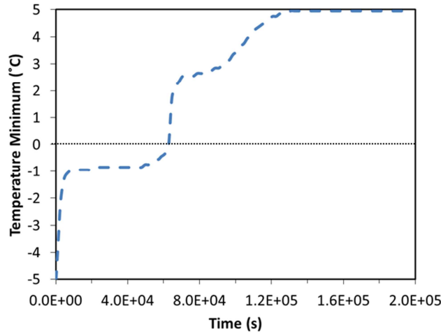
Fig. 3 Evolution of the minimum temperature with time using 1134 elements.
