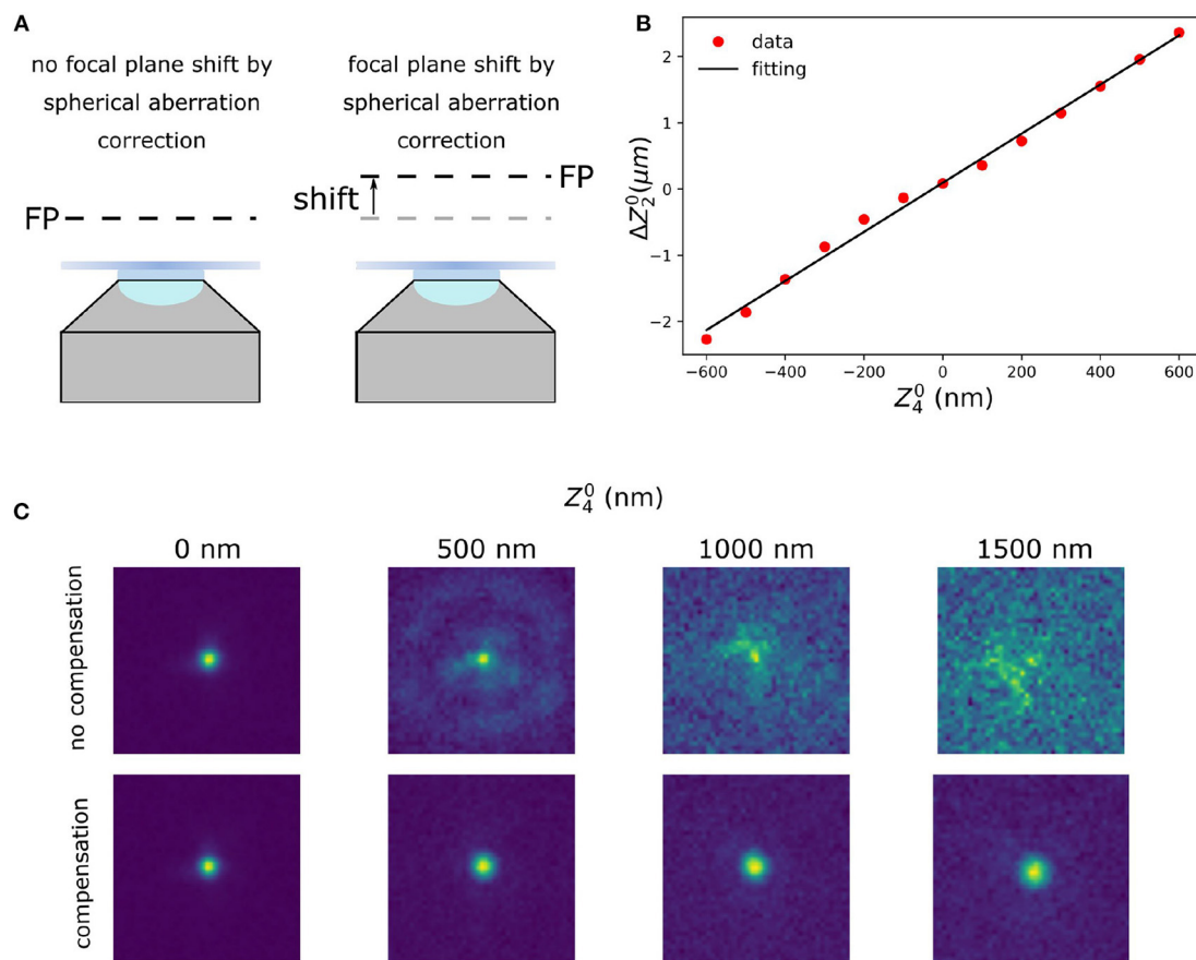
FIGURE 2 Defocus calibration for spherical aberration compensation. (A) Focal plane shift induced by coupling between defocus and spherical aberration. When correcting for the spherical aberration, the coupling between the spherical and the defocus aberration shifts the focal plane (FP). (B) Calibration of the compensation for the defocus introduced by spherical aberration. (C) Raw data with different amount of spherical aberration ( Z_4^0 : 0, 500, 1,000, and 1,500 nm) without (upper row) and with (lower row) defocus compensation. The calibration was done with spherical aberration in the range of -600 \sim 600 nm.
