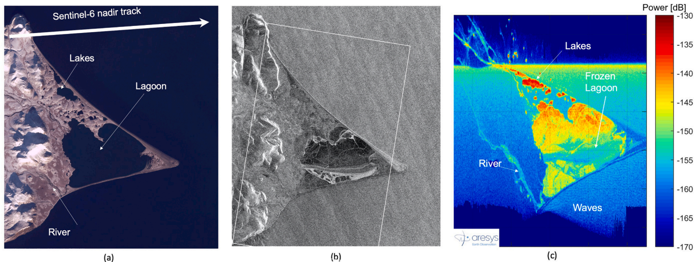
Fig. 17. (a) Sentinel-2B colour composite image of Ozero Nayvak peninsular (64.433 N, -172.3466 W), Russia obtained on 15th August 2020 with annotations of key features. (b) Sentinel-1b interferometric wide-swath C-band SAR image obtained on 29th November 2020. (c) S6-MF fully-focussed SAR (FFSAR) image obtained on November 30th 2020 processed by Aresys. The FFSAR image is not geolocated or projected and the white square indicates the approximate position of the Sentinel-6 altimeter image in (c).
