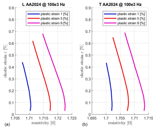
Fig. 4. Piezoresistivity curves for various amounts of plastic strain for aluminum 2024-T3: (a) longitudinal grain, (b) transverse grain. Note initial nonlinearity with increasing strain.
