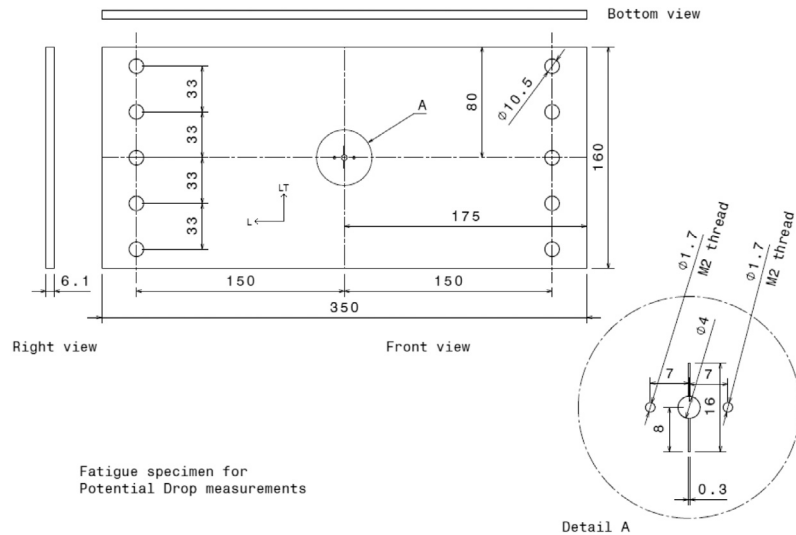
Fig. 7. Drawing of a typical fatigue test specimen as used with the PD TTC setup. Loading direction horizontal. The constant current was connected through the edge holes on the horizontal centerline.
