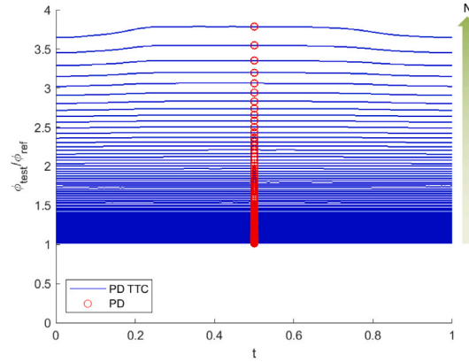
Fig. 9. Potential ratio curves of test 1, per cycle time t . A subset consisting of each 250th curve is shown for clarity. With increasing crack length, the ratio increases. The values at t = 0.5 correspond to standard S_{\max} PD values.
