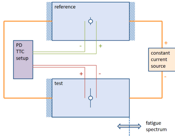
Fig. 5. Schematic view of the test setup with potential drop measurement device and constant current source. Actual tests were performed with a 250 kN MTS fatigue machine.
