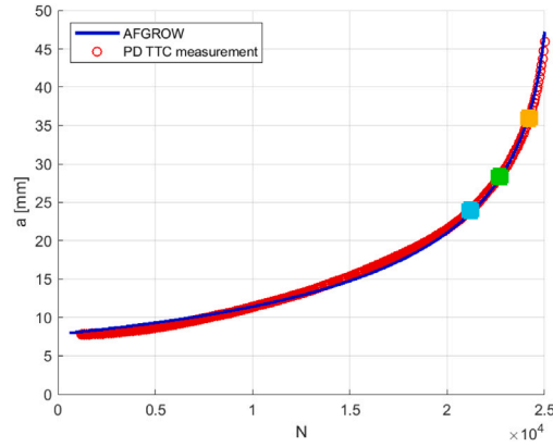
Fig. 10. Crack length versus cycles for test 1. Red data points are generated using the method given in ASTM E647 [9], using the potential values at t = 0.5 from the curves shown in Fig. 9. AFGROW curve shown for comparison. The orange, green, and cyan markers correspond with the points in Fig. 11 and curves in Fig. 12.
