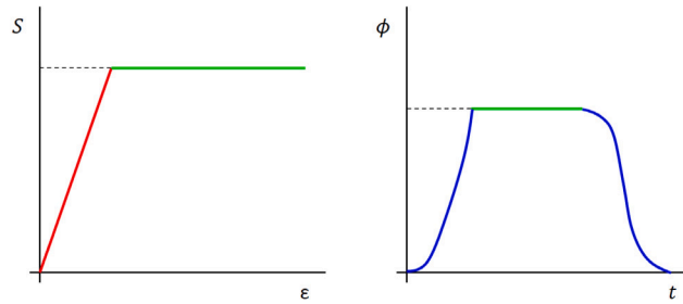
Fig. 16. Elastic perfectly plastic stress–strain curve and corresponding schematic PD TTC curve. Above a certain stress level near or at S_{yield} , plastic deformation exists, which increases \epsilon at constant stress and constant potential, resulting in a plateau (green).
