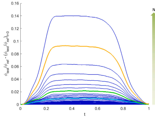
Fig. 12. Potential TTC curves of test 1, per cycle time t . These are the same curves as in Fig. 9, now translated vertically to start from zero to facilitate comparison of the PD TTC curve shape. The orange, green, and cyan curves correspond with the similarly colored points in Figs. 10 and 11.
