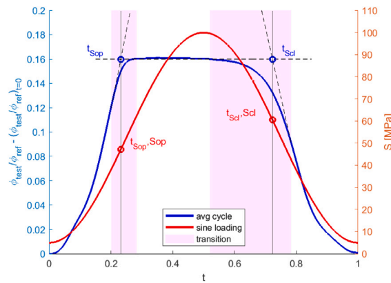
Fig. 17. The plateau region has a nearly constant potential, showing a balanced act between the Poisson effect and the piezoresistivity. Crack opening and closure transition time intervals shown in magenta.
