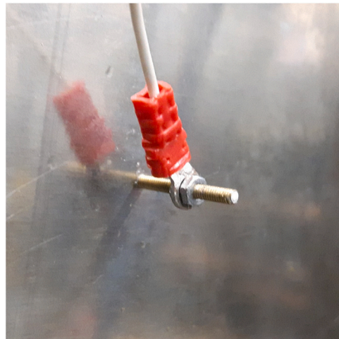
Fig. 8. Close-up of a representative PD electrode attachment. The M2 brass bolt connects the PD wire with the specimen.
