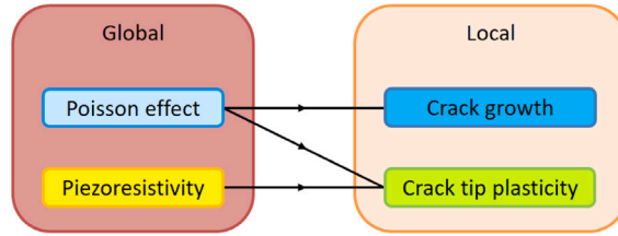
Fig. 3. A schematic view of how the global and local PD effects are related.
