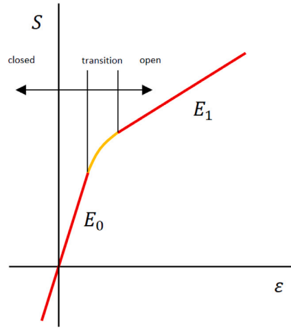
Fig. 18. A schematic, global stress-strain diagram of the specimen belonging to Fig. 17. The nonlinear section (orange) relates to the transition from a closed crack ( E_0 ) to an open crack ( E_1 , PD TTC plateau).
