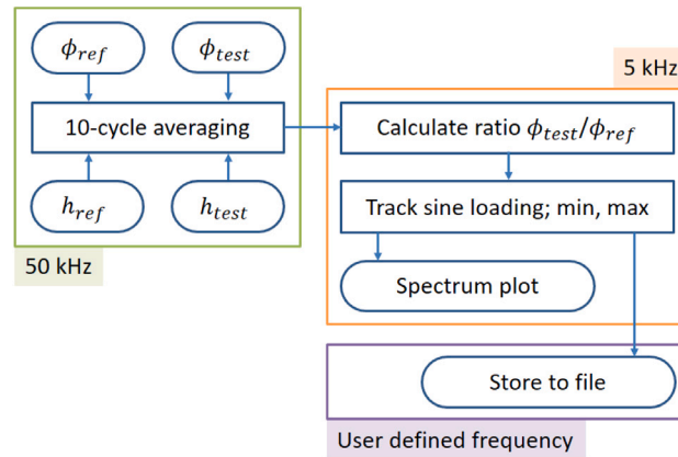
Fig. 6. Potential drop measurement FPGA flow chart.
