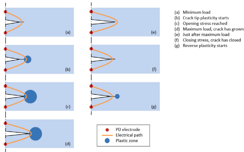
Fig. 1. Schematic view of the PD measurement electric path through a fatigue specimen, at several stages during a fatigue cycle. The applied current flows vertically in each stage.
