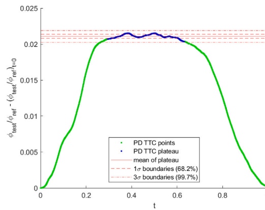
Fig. 14. Potential TTC curve of test 1, corresponding to the green curve in Fig. 12. The plateau data is shown in blue, with 1\sigma and 3\sigma standard deviation bands.
