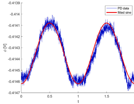
Fig. 15. Two PD TTC cycles from test 8, with an overlaid sine curve representing the applied loading. A clear correlation is observed throughout the cycles. Compare with Fig. 12; the plateau only appears when crack tip plasticity is present.
