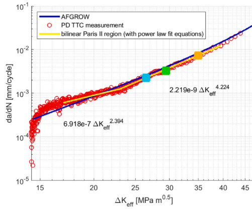
Fig. 11. Crack growth rate curve of test 1. A bilinear Paris region II is observed in the range 17 < \Delta K_{\text{eff}} < 40 . AFGROW curve shown for comparison. The orange, green, and cyan markers correspond with the points in Fig. 10 and curves in Fig. 12.
