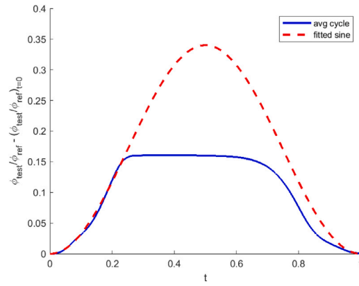
Fig. 13. A single TTC curve from measurements, with an overlaid sine curve representing the applied loading. A correlation is observed during the first and last quarter of the cycle. A plateau appears in between, at a certain load level.
