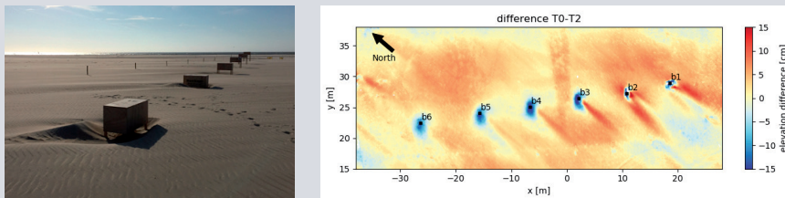
Figure 3 (left) and 4 (right). Final photo and elevation difference map of the beach group - in red the concentrated local deposition (up- and downwind) around the non-elevated boxes (B1, B2); versus local erosion (in blue) and dispersed tails around the boxes with increasing pole-height (B3 (+25cm) - B6 (+1m))
