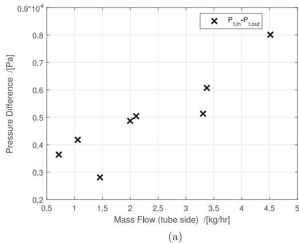
Fig. 17. Pressure drop over the mini-channel heat exchanger on the tube side (NH 3 -CO 2 -H 2 O side) (a), and the shell side (water side) (b).
