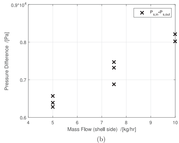
Fig. 17. Pressure drop over the mini-channel heat exchanger on the tube side (NH 3 -CO 2 -H 2 O side) (a), and the shell side (water side) (b).
