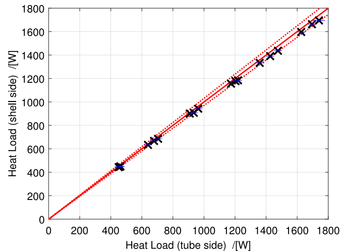
Fig. 14. The heat load on the shell and tube sides for the \text{NH}_3\text{-H}_2\text{O} experiments. The difference is within 3% (dotted line) for all the experiments.
