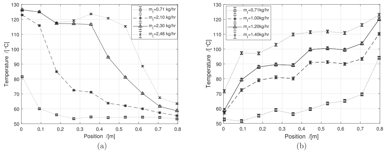
Fig. 23. Temperature results from the sensors located along the shell side of the mini-channel heat exchanger for a shell side mass flow of 5 kg/h, for absorption in downward flow of the \text{NH}_3\text{-CO}_2\text{-H}_2\text{O} mixture (a), and in upward flow of the \text{NH}_3\text{-CO}_2\text{-H}_2\text{O} mixture (b). Error bars are included (see Section 2 for details). The lines serve as visual guidelines for the reader.
