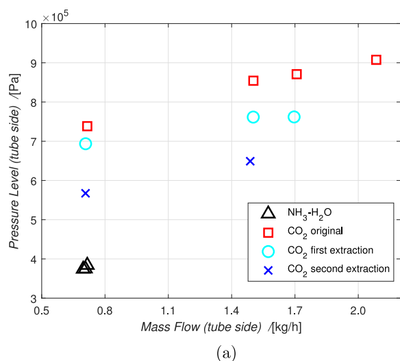
Fig. 21. Results for a shell side mass flow of 5 kg/h before and after draining of the mixture with added CO 2 compared to the NH 3 -H 2 O results, the different pressure levels (a), and the shell side heat load (b). It is clear that comparable pressure levels were not reached with the added CO 2 . However, with each extraction the performance at similar mass flows approached the performance of the NH 3 -H 2 O mixture.
