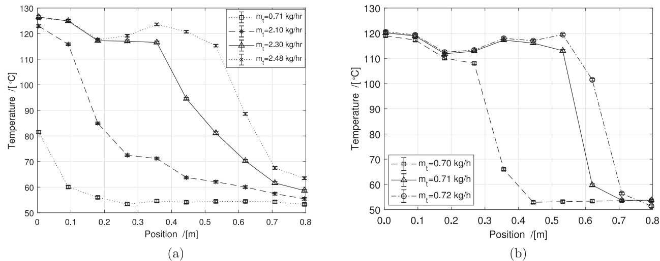
Fig. 22. Temperature results from the sensors located along the shell side of the mini-channel heat exchanger for a shell side mass flow of 5 kg/h, for the \text{NH}_3\text{-CO}_2\text{-H}_2\text{O} mixture (a), and the \text{NH}_3\text{-H}_2\text{O} mixture (b). Error bars are included (see Section 2 for details). The lines serve as visual guidelines for the reader.
