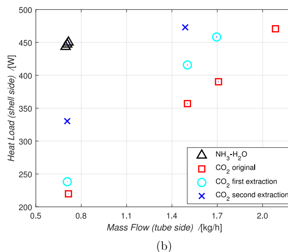
Fig. 21. Results for a shell side mass flow of 5 kg/h before and after draining of the mixture with added CO 2 compared to the NH 3 -H 2 O results, the different pressure levels (a), and the shell side heat load (b). It is clear that comparable pressure levels were not reached with the added CO 2 . However, with each extraction the performance at similar mass flows approached the performance of the NH 3 -H 2 O mixture.
