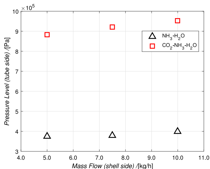
Fig. 20. Pressure levels for the NH 3 -H 2 O and NH 3 -CO 2 -H 2 O experiments for shell side mass flows of 5, 7.5 and 10 kg/h.
