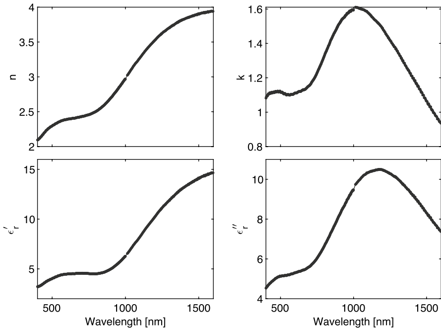
Fig. 4 Optical constants ( n,k ) and relative permittivity for TiN. These values are derived from a multi-angle spectroscopic ellipsometry measurement of a 60-nm thick TiN film deposited on a 350 \mu\text{m} polished c-plane sapphire substrate. Individual measurements points are plotted, showing a gap around 1000 nm where the set-up switches between two different detectors. Measured from 191.35 to 1688.0 nm in 710 non-equidistant measurement points.
