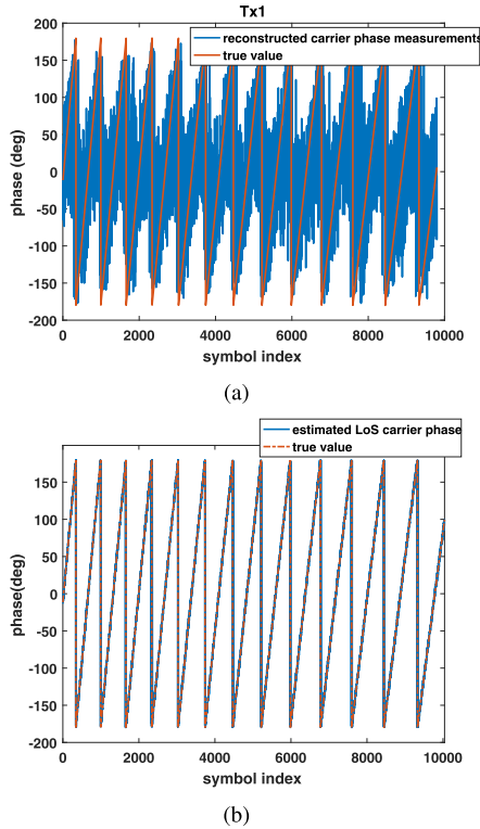
FIGURE 10. ‘Vehicular A’ multipath channel with SNR = 20 dB, (a) carrier phase derived based on phase combination of two symmetrically located subcarriers (e.g., (+/-12) -th subcarrier) [34]; (b) LoS carrier phase estimated from proposed two-step approach.
