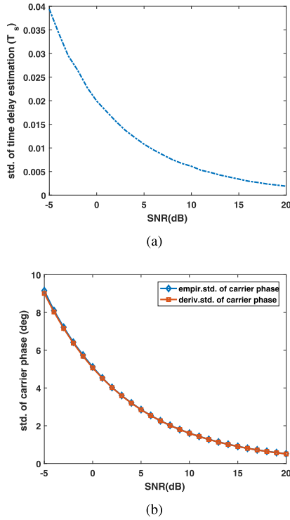
FIGURE 7. (a) Empirical standard deviation of time delay \sigma_\delta and (b) both the empirical and derived standard deviation \sigma_\phi (46) of carrier phase estimation versus SNR.
