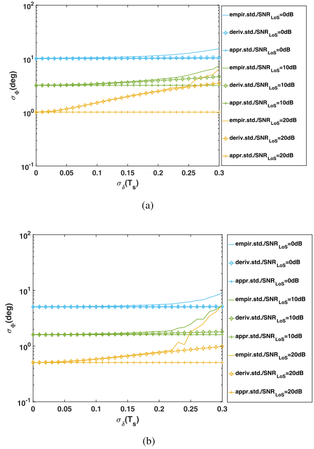
FIGURE 6. (a) Using only N_p = 16 pilot subcarriers with a spacing of \Delta p = 4 and (b) using all subcarriers N = N_p = 64 with a spacing of \Delta p = 1 (b), standard deviation of carrier phase estimation error \sigma_\phi versus standard deviation of time delay error \sigma_\delta (in units of T_s ) for three different SNRs 0, 10, and 20 dB, in which ‘ empir.std. ’ denotes the empirical standard deviation computed from the simulation, ‘ deriv.std. ’ denotes the theoretical standard deviation derived from (45), and ‘ appr.std. ’ denotes the approximation of the standard deviation in (46).
