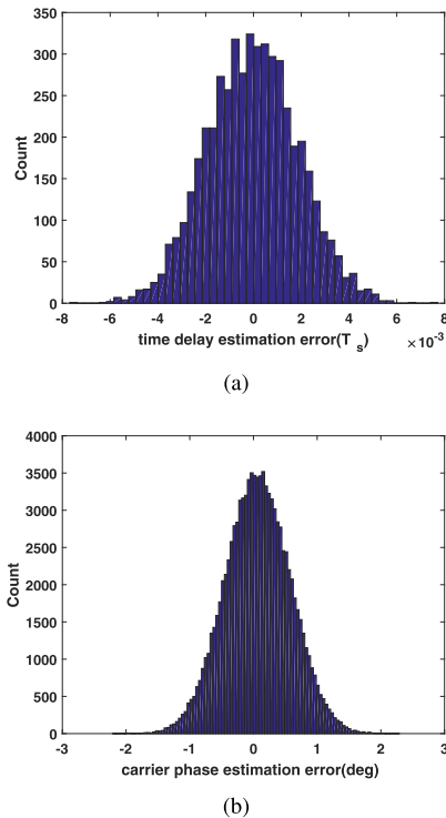
FIGURE 8. (a) histogram of ESPRIT-based time delay error as SNR = 20dB, (b) histogram of carrier phase estimation error as SNR = 20dB.
