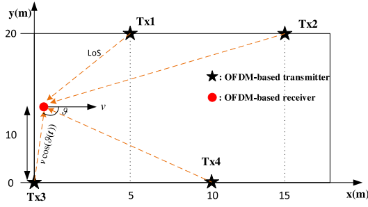
FIGURE 1. A 2-D roadway positioning scenario: four transmitters with fixed and known locations and one rover receiver moving with a speed of v , indicated by the black arrow.
