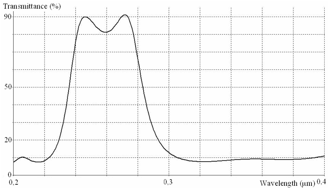
Figure 3: Simulation of the transmittance versus wavelength of a UV bandpass optical filter with 11 layers (composed of \text{Y}_2\text{O}_3 , \text{TiO}_2 and \text{SiO}_2 ).
