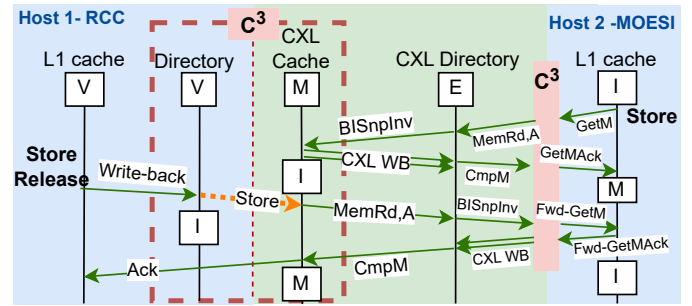
Fig. 8: Example operations with RCC-CXL Bridge. The C^3 instance for host 2 is simplified for brevity.
