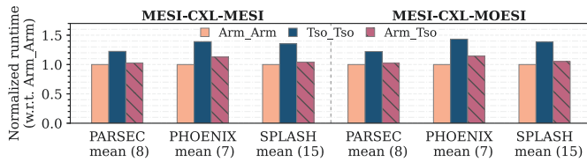
Fig. 9: Performance comparison of heterogeneous MCMs in two scenarios: homogeneous and heterogeneous CC protocols.
