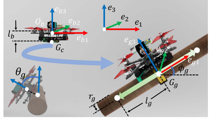
Fig. 4. Modeling overview and symbols definition.
