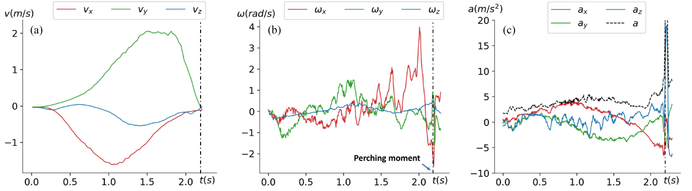
Fig. 8. Flight data of agile perching on 40° angled branch: (a) Ground truth velocities are zero at hover state ( t = 0 s) and prior to the perched state ( t \approx 2.2 s), (b) body rate, and (c) accelerations of the drone measured onboard.
