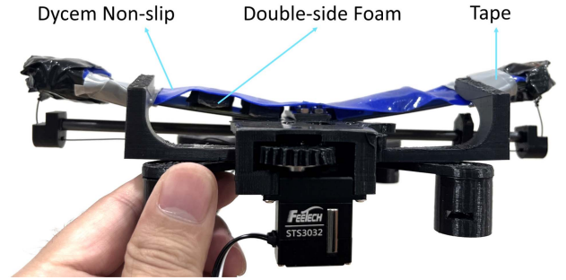
Fig. 3. Gripper mechanism for agile quadrotor perching.
