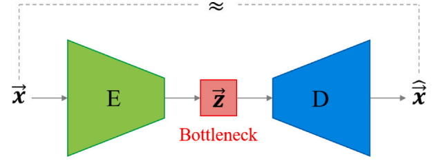
Fig. 1. Typical architecture of an AE: E is the Encoder, and D is the Decoder.
