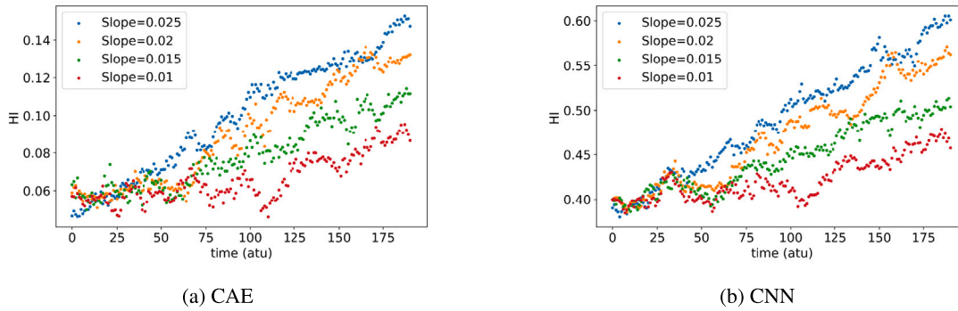
Fig. 12. Linear degradation with varying slopes — HI corresponding to (a) the proposed CAE trained by the hybrid algorithm and (b) the equivalent CNN.
