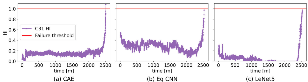
Fig. 24. Bearing B31 HIs based on the three models.
