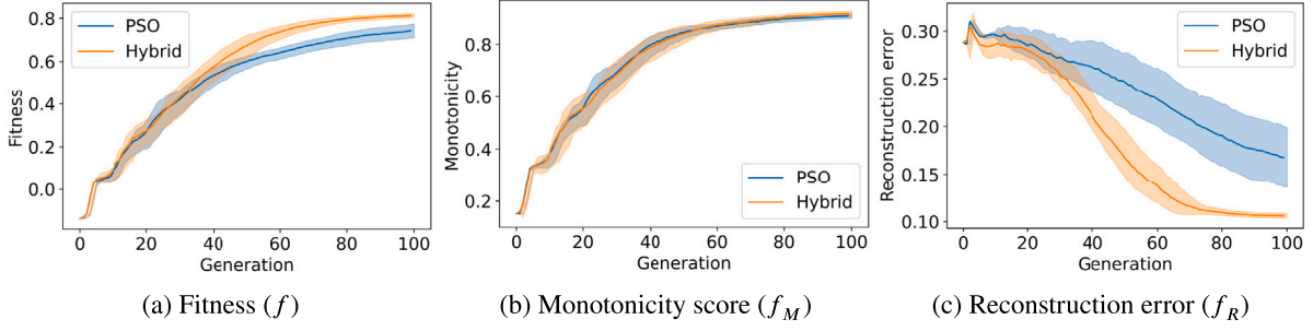
Fig. 7. \text{mean} \pm \text{std} of fitness, monotonicity score, and reconstruction error of the best particle in each generation.
