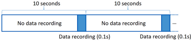
Fig. 13. PHM 2012 vibration data recording scheme.
