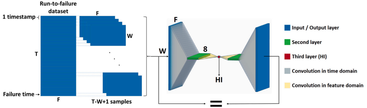
Fig. 2. CAE architecture.
