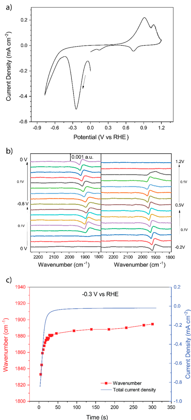
Figure 7. (a) Cyclic voltammetry curve of SEIRA active Pd thin films between -0.8 and 1.2 V in \text{CO}_2 saturated \text{KHCO}_3 solution. Scan rate: 10 mV/s. (b) Recorded in situ SEIRA spectra of adsorbed CO during the acquisition of the voltammetry curve. (c) Current transient of SEIRA active Pd films and peak center of CO peak at an applied potential of -0.3 V vs RHE in \text{CO}_2 saturated \text{KHCO}_3 solution.
