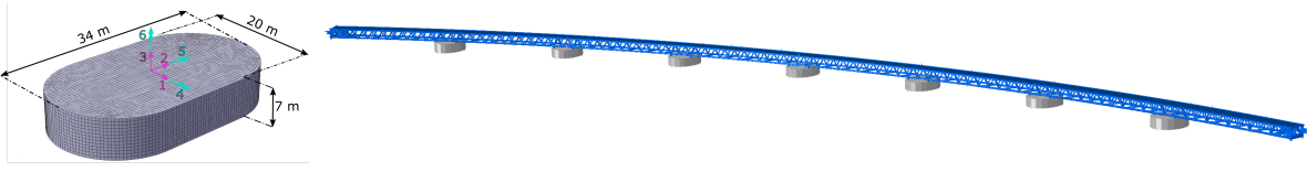
Figure 3: Left: HydroD model of a pontoon; right: ABAQUS model of the bridge.
