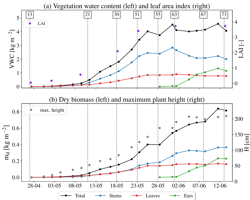
Fig. 5. Seasonal pattern of (a) vegetation water content ( \text{kg m}^{-2} ) per constituents and leaf area index, and (b) dry biomass ( \text{kg m}^{-2} ) per constituents and canopy height (cm). Phenological stages are shown by BBCH codes, which are explained in Table 2. (For interpretation of the references to color in this figure legend, the reader is referred to the web version of this article.)
