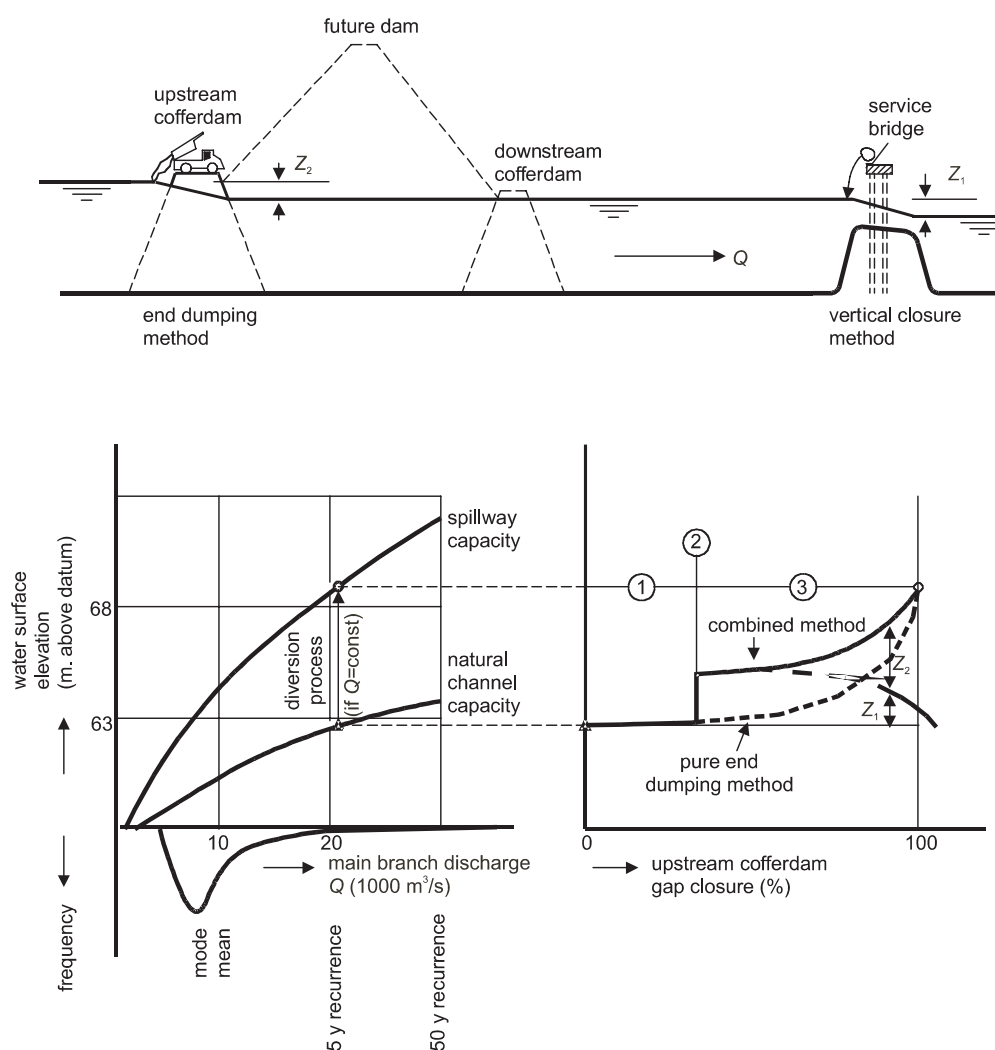
Figure 7.21 Yacycrta diversion scheme, River Paraná, Argentina
