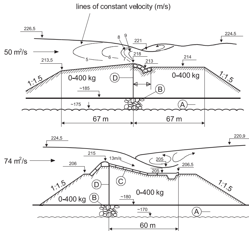
Figure 7.22 Cross-section over upstream and downstream cofferdams (D) at Cabora Bassa, Mozambique (dimensions in m) – units per metre width
