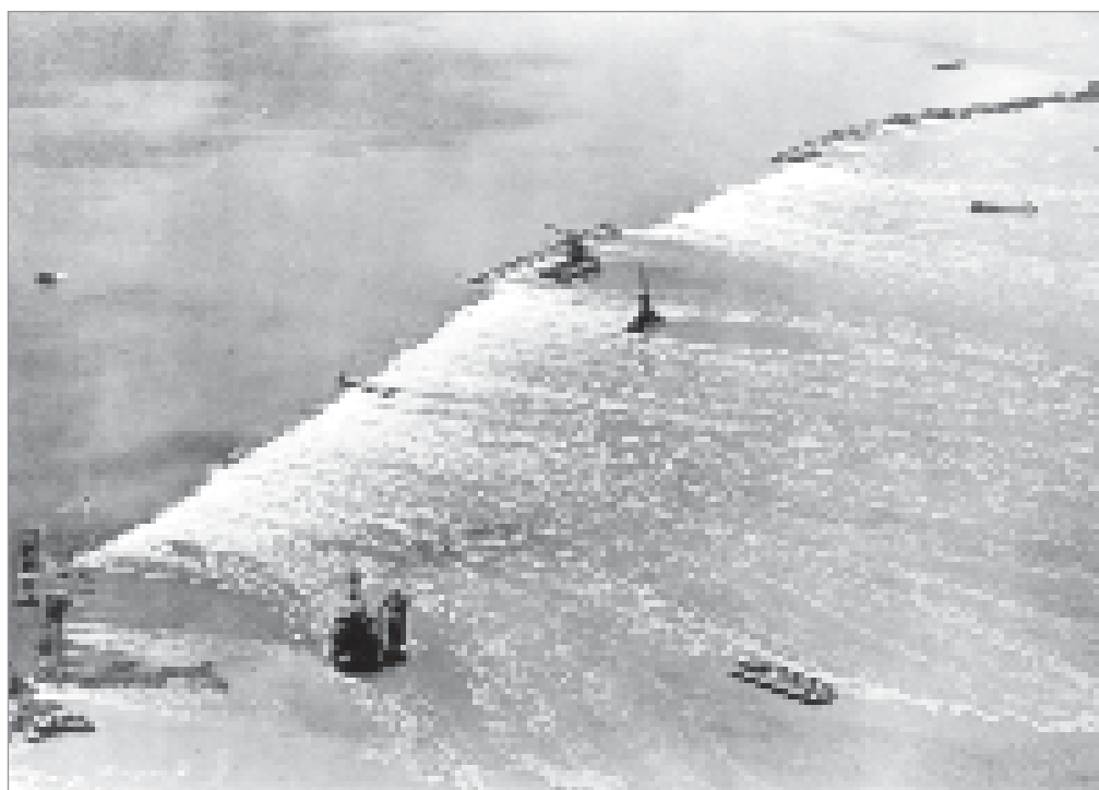
Figure 7.30 Bed protection in Schelphoek shallow closure, the Netherlands (1953) (courtesy KLM)
