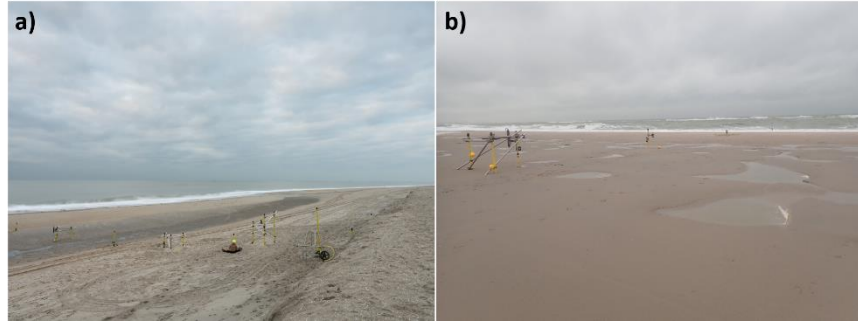
Fig. 2. 3D complexities formed during calmer conditions between storms, such as crescentic bars (a, taken on Nov 27) and mega-ripples (b, taken on Dec 3)
