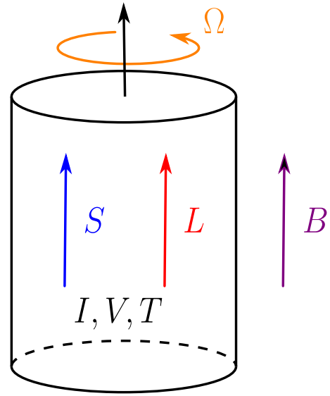
FIG. 2. The system under consideration in Sec. III: A macroscopic ferromagnet with moment of inertia I and volume V at temperature T . The total spin S of the ferromagnet is aligned parallel to an external magnetic field B . In addition, the ferromagnet may rotate with angular velocity \Omega and supports a phonon spin L . The system is assumed to be at rest with \Omega = 0 initially. Finite \Omega and L are induced by exciting the system into a nonequilibrium state at time t = 0 , e.g., by heating the phonons or by pumping the magnons with an rf field. In this case both \Omega and L are parallel to the total spin S because of the conservation of total angular momentum.
