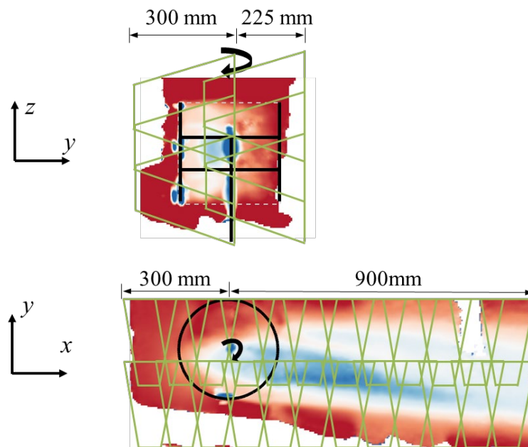
Figure 3. Measurement views in the horizontal ( X - Y ) and vertical ( Y - Z ) plane.
