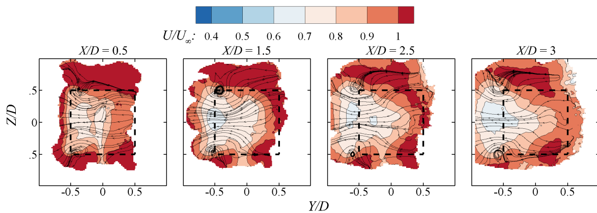
Figure 7. Stream-wise velocity contours and in-plane streamlines at cross-sections downstream of the VAWT rotating in TSR of 1.5 ( X/D = [0.5, 1.5, 2.5, 3] ).
