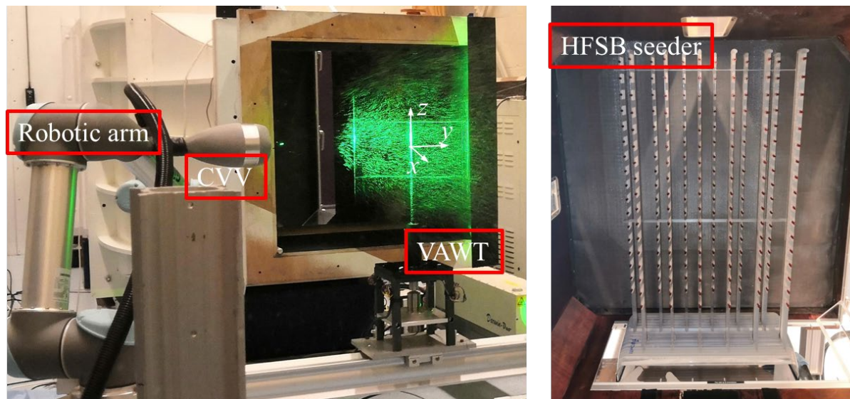
Figure 1. Experimental set up: Robotic PIV measuring (left), HFSB seeder inside the settling chamber of W-tunnel (right).
