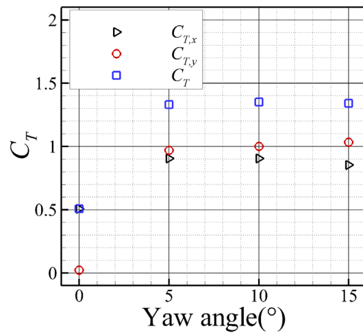
Figure 5. The time-averaged streamwise, lateral and overall thrust coefficients of porous plates vary with yaw angle.
