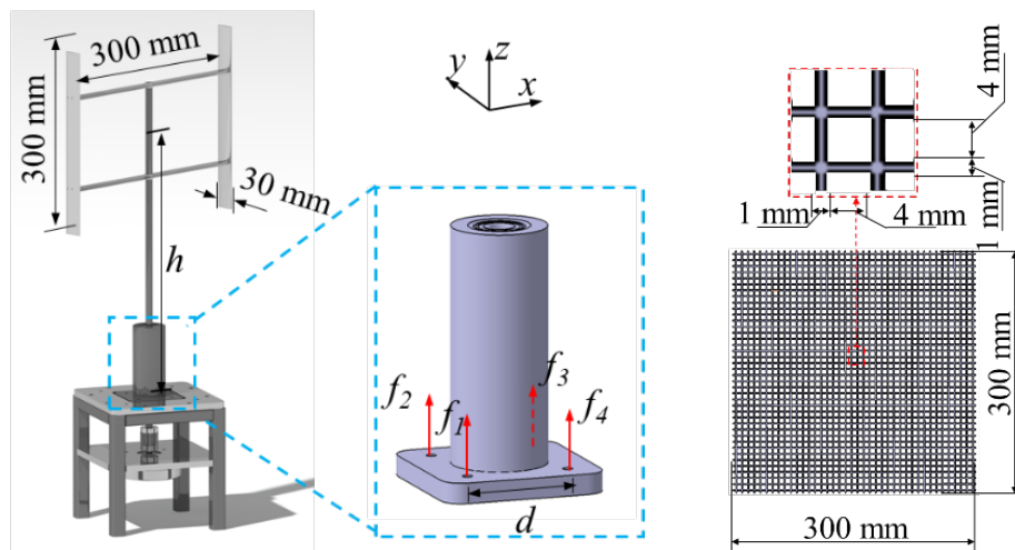
Figure 2. Schematic plotting of the models: VAWT model with a thrust measurement system (left) and porous plates (right).
