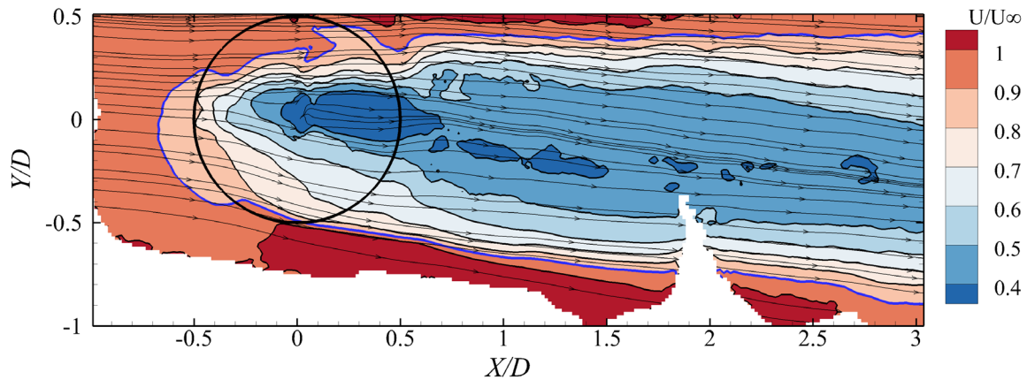
Figure 12. Time-averaged and normalized stream-wise velocity contour and streamlines in the XY -plane along with the streamline, Z/D = 0 , \lambda = 2.5 .
