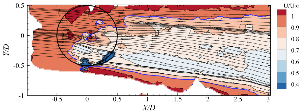
Figure 11. Time-averaged and normalized stream-wise velocity contour and streamlines in the XY -plane along with the streamline, Z/D = 0 , \lambda = 1.5 .
