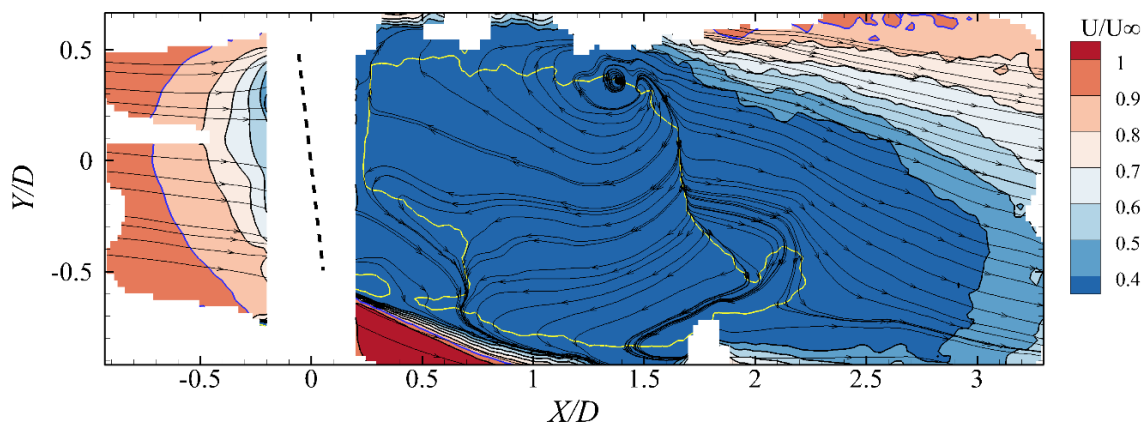
Figure 13. Time-averaged and normalized stream-wise velocity contour and streamlines in the XZ -plane at Y/D = 0 .
