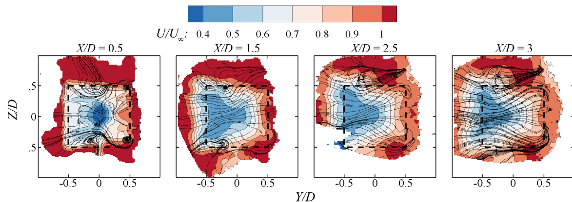
Figure 8. Stream-wise velocity contours and in-plane streamlines at cross-sections downstream of the VAWT rotating in TSR of 2.5 ( X/D = [0.5, 1.5, 2.5, 3] ).
