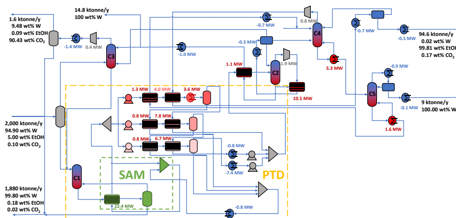
Figure 3. Flowsheet of bioethanol recovery process, PTD-MED configuration
