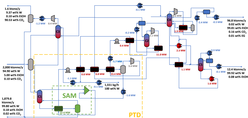
Figure 2. Flowsheet of bioethanol recovery process, PTD-HP configuration
