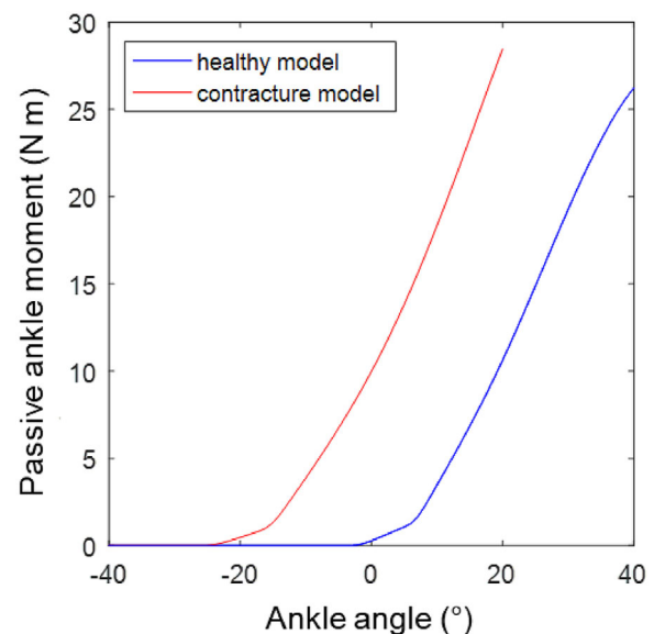
FIGURE 1 The passive ankle moment–ankle angle curve for the healthy, default model and for the pathology-specific contracture model representative for idiopathic toe walkers, with a shift of 20°. For the contracture model, the optimal fibre lengths and tendon slack length were obtained by minimising the root mean square error between the gastrocnemius and soleus passive moment–angle curve of the model and the 20° shifted curve
