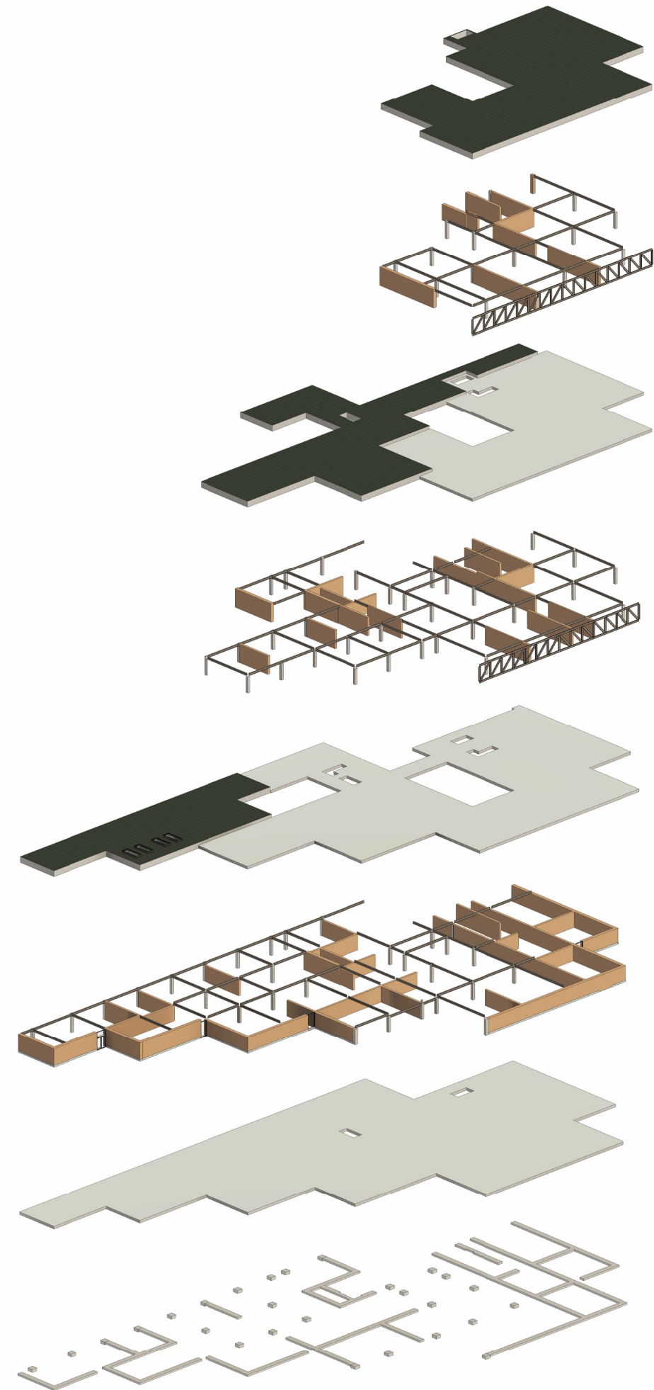
Slim floor (Prefab+in-situ cast concrete)
