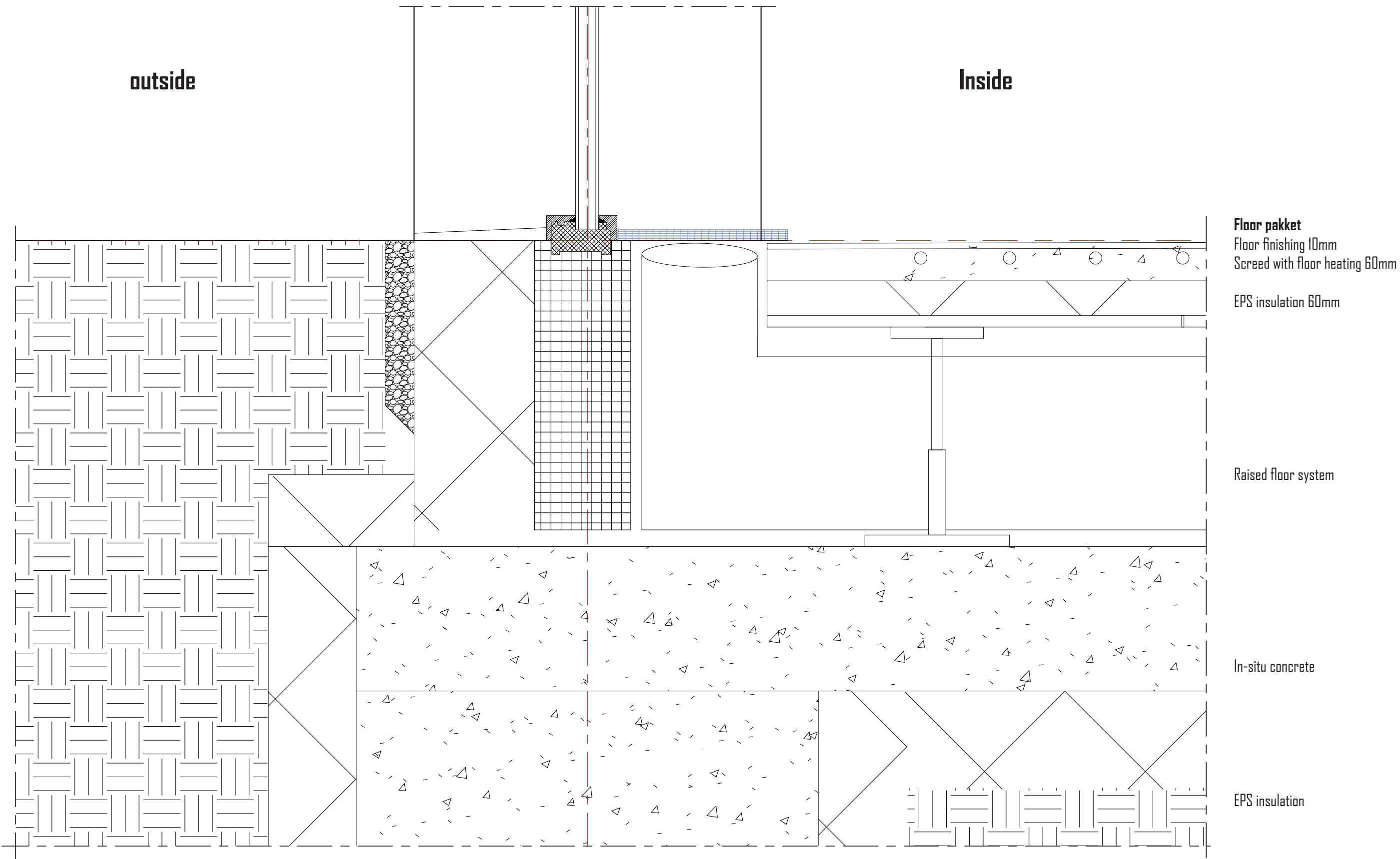
Foundation detail 1:5 (rescaled) Design proposal
