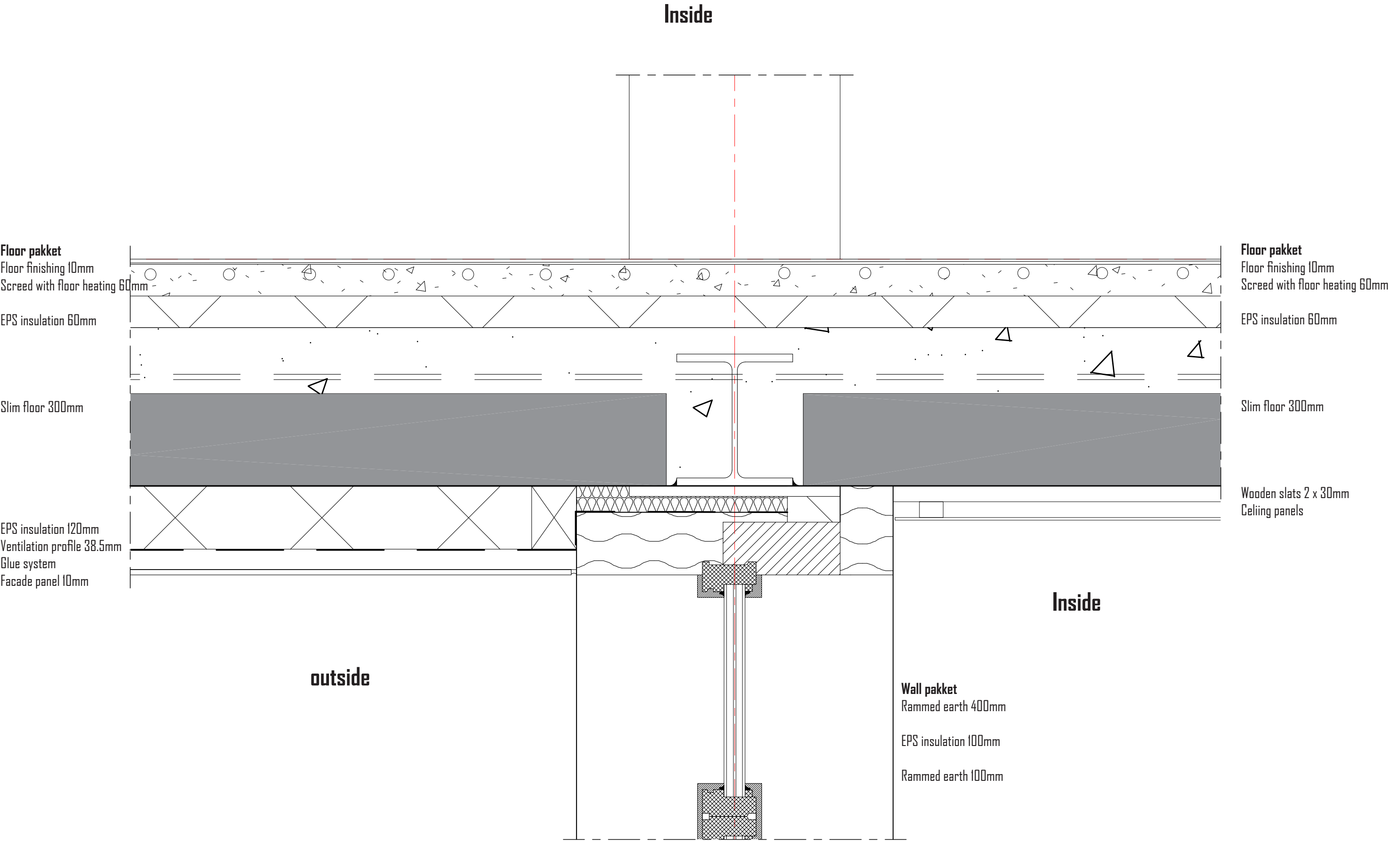
Connection floor to wall detail 1:5 (rescaled) Design proposal
