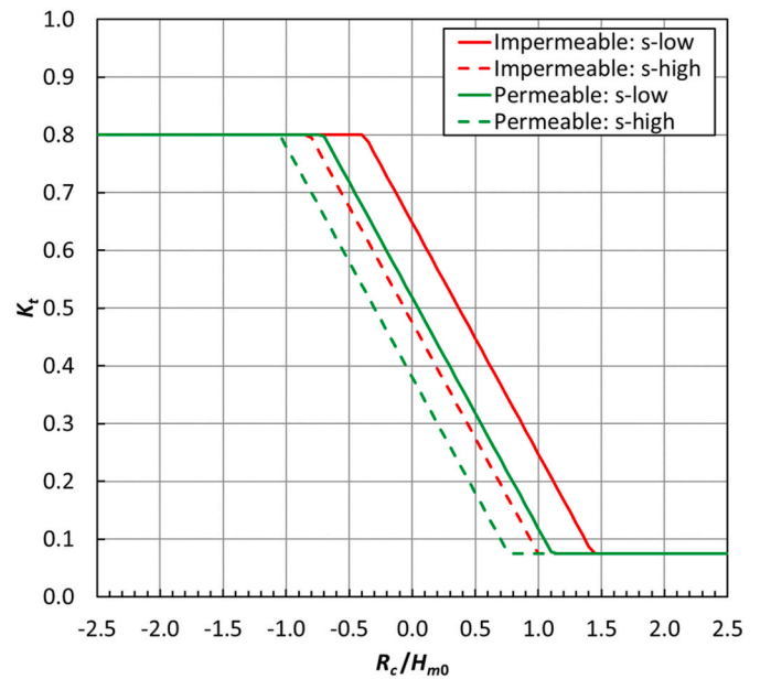
Fig. 2. Wave transmission as function of the non-dimensional freeboards as expressed by d'Angremond et al. (1996) for impermeable and permeable structures (1:2 slopes and crest width of B/H_{m0} = 1.5 ).
