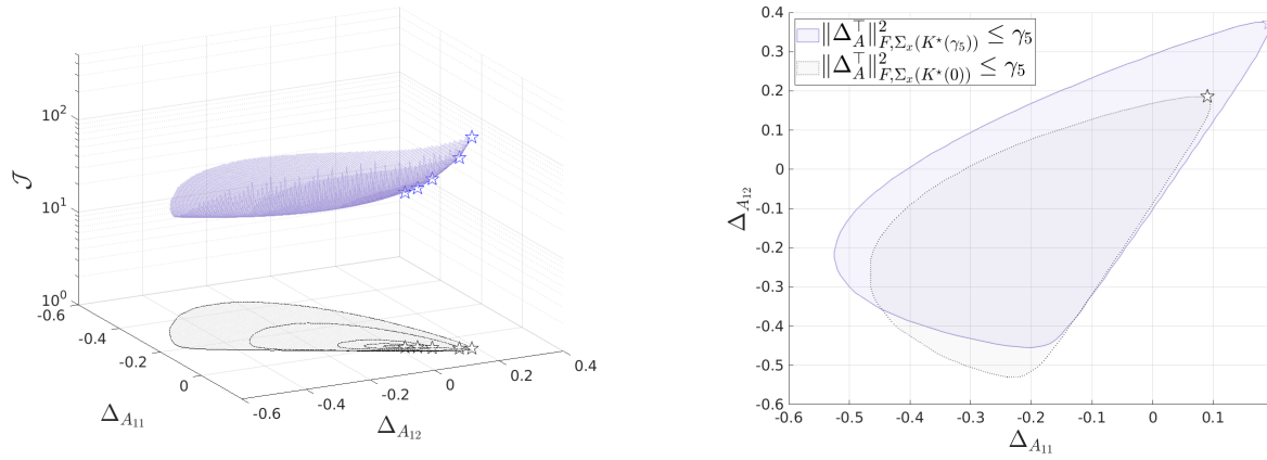
(a) For \gamma \in \Gamma , the sets \Delta_\gamma(\hat{A} + BK^*(0)) with the corresponding worst-case path, including a projection on the cost surface. (b) Comparison of the uncertainty hedged against for the nominal-, K^*(0) , and robust controller K^*(1) , i.e., \Delta_{\gamma=1} under both K .
