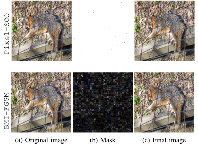
Fig. 2: Pixel-SOO vs. BMI-FGSM results for Image ‘ILSVRC2012_val_00000323.JPEG’
